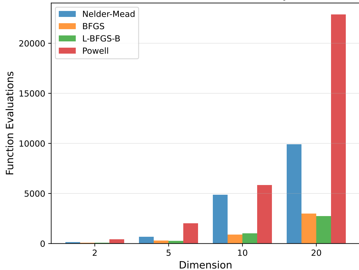
Rosenbrock: Function Evaluations by Method
