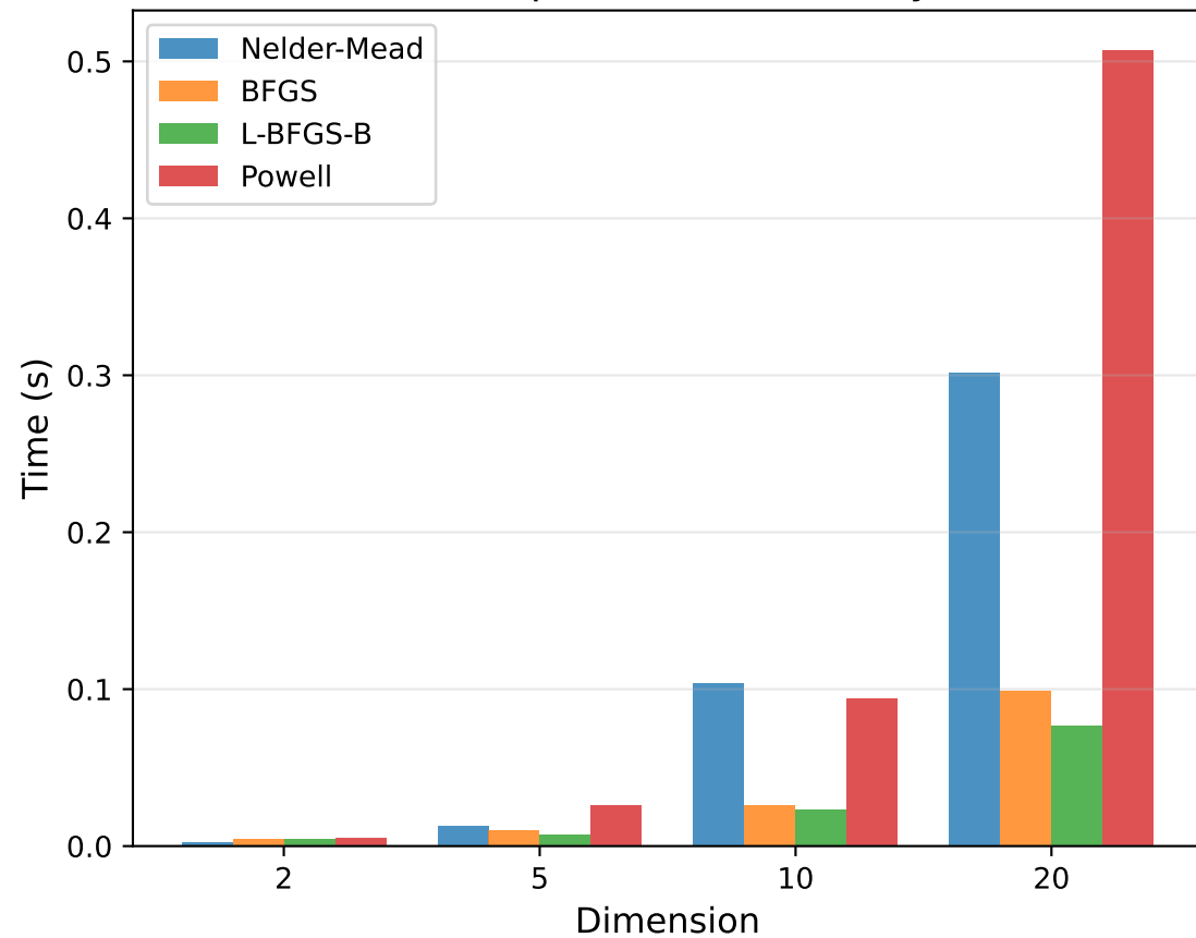
Rosenbrock: Optimization Time by Method
