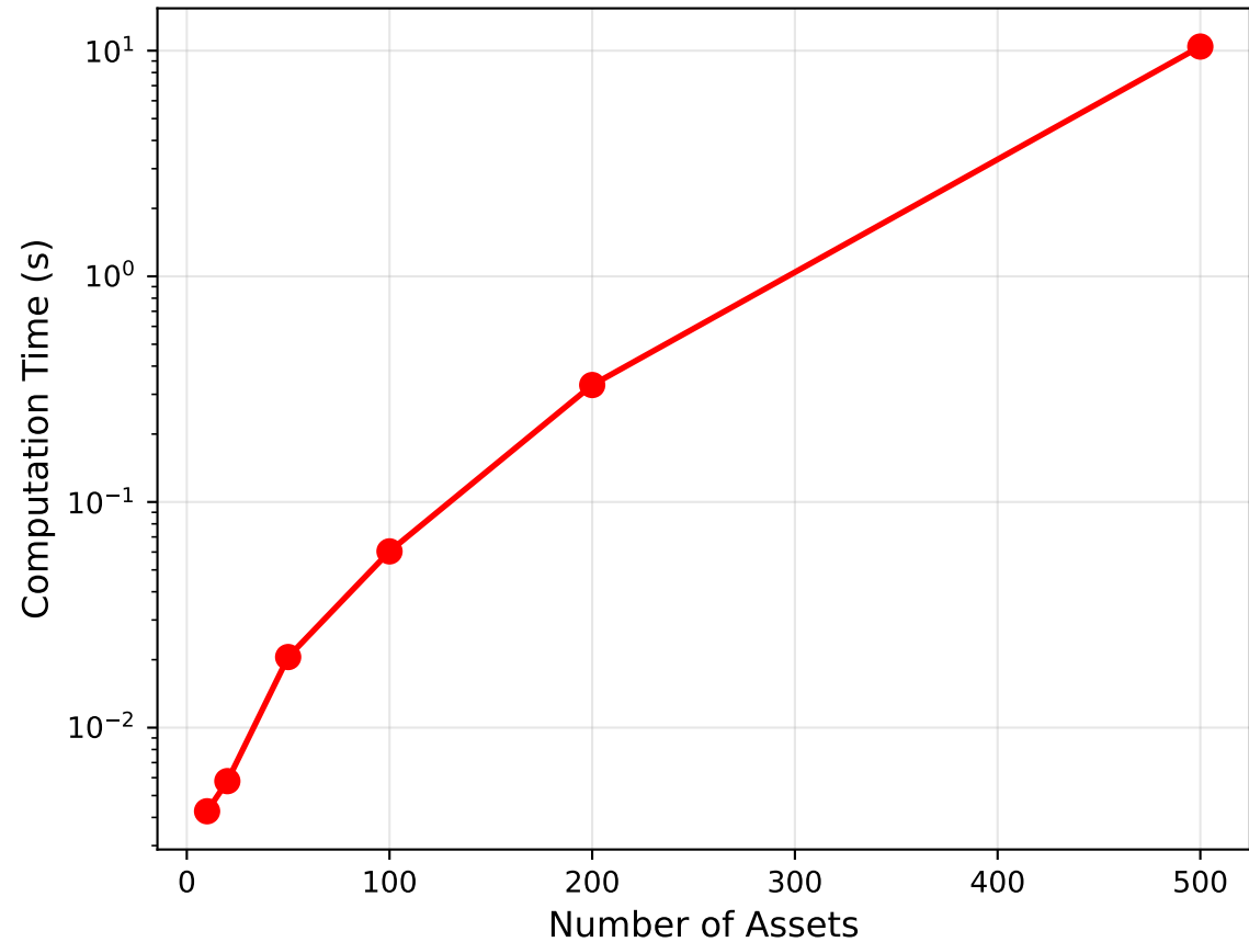
Portfolio Optimization: Time Complexity
