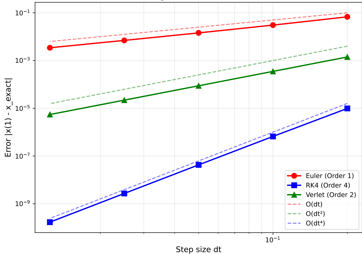
Convergence Order Verification
