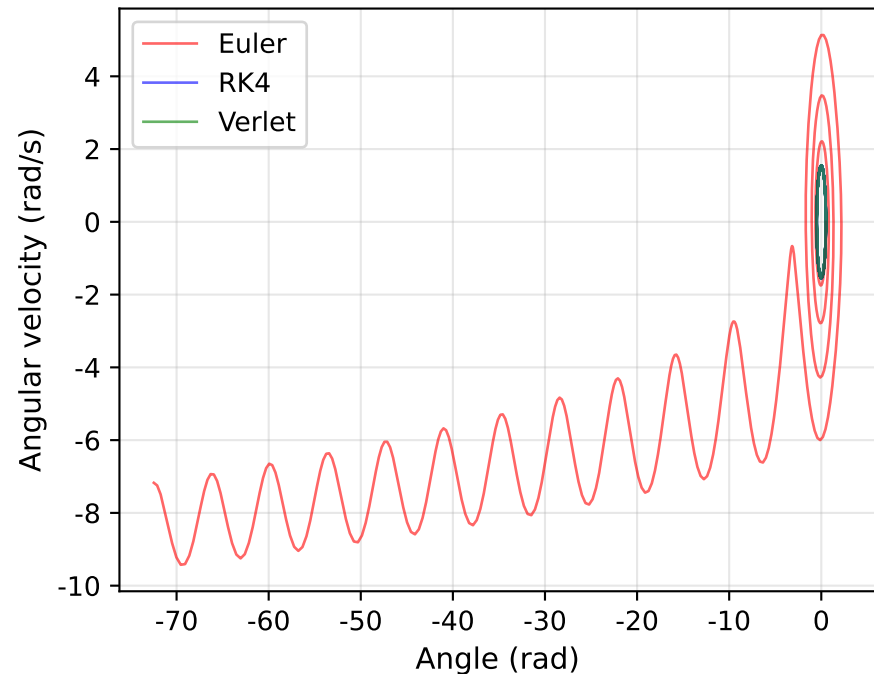
Phase Space
