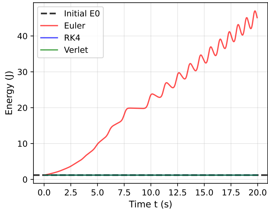
Energy Conservation
