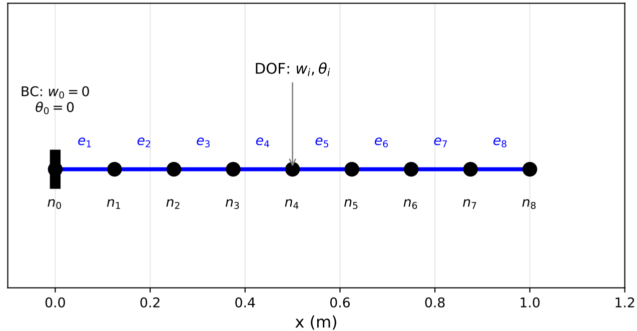
FEM Mesh: Euler-Bernoulli Beam Elements
