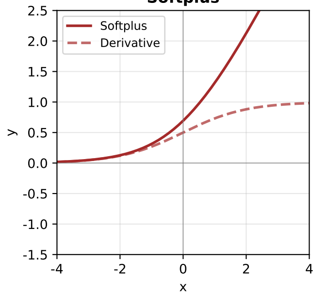
Softplus
