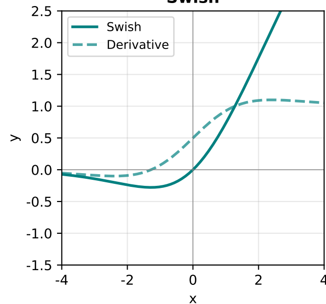
Swish
