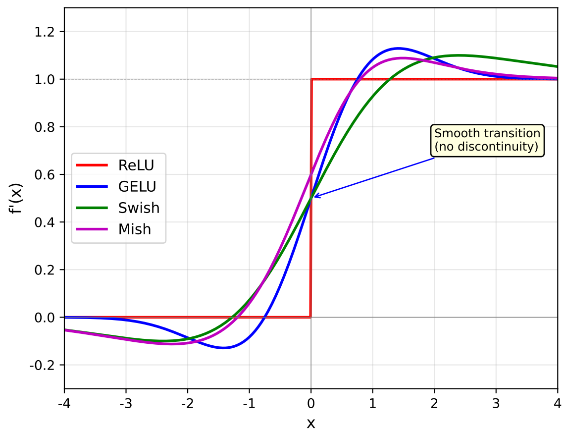
Derivatives of Modern Activations
