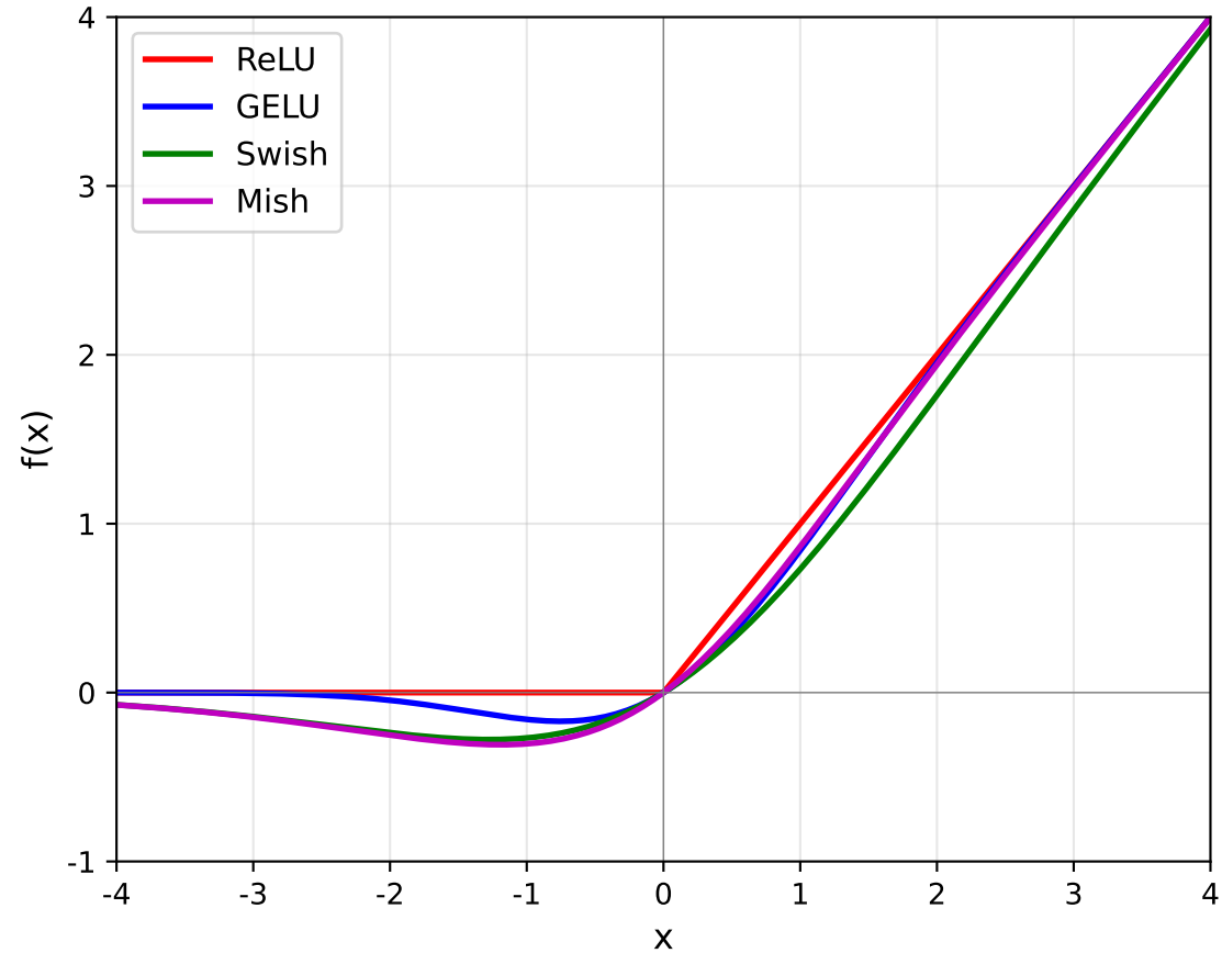
Modern Activation Functions
