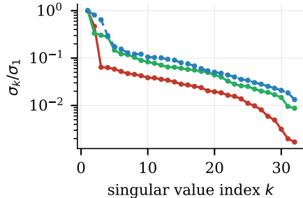
(c) spectrum of Cov(z)
