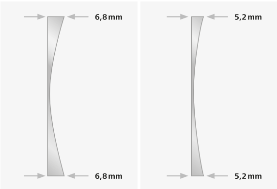
Mineral 1.6 (left) compared to mineral 1.8 (right), -7.0 D and @ 70 mm of illustrated lenses.
