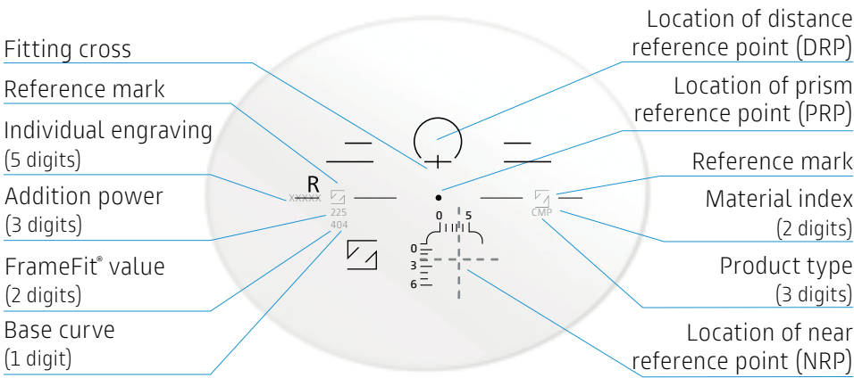
ZEISS Progressive ClearMind Plus / Superb lens
