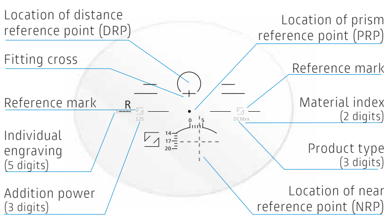
ZEISS Digital ClearMind Lenses lenses
