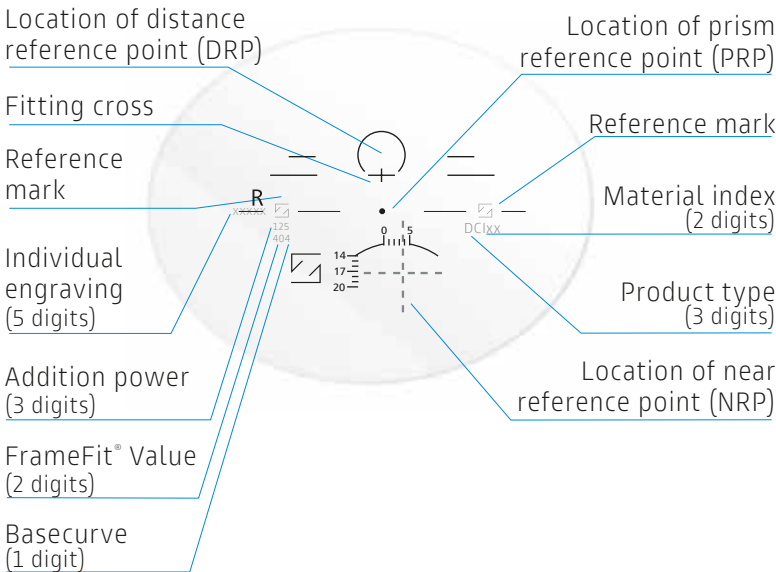
ZEISS Digital ClearMind Individual 3 Lenses
