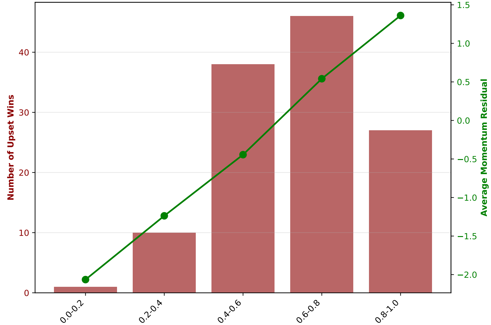
Upset Wins and Momentum by Finish Position
