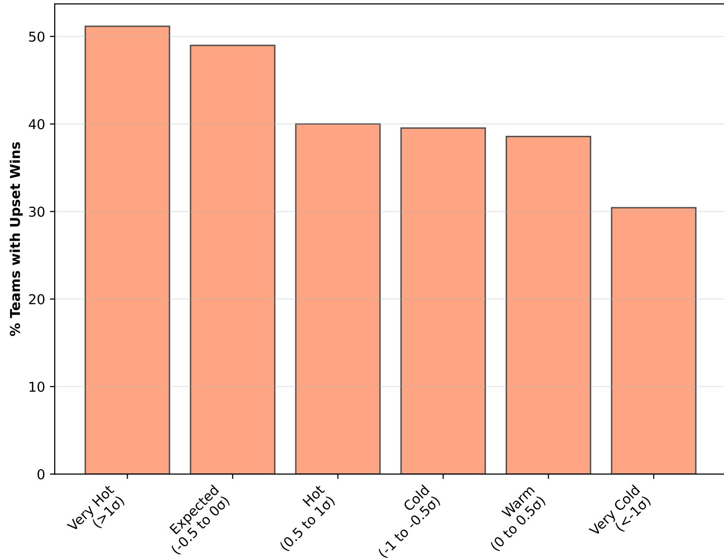
Momentum Distribution: Upset Winners vs Others
