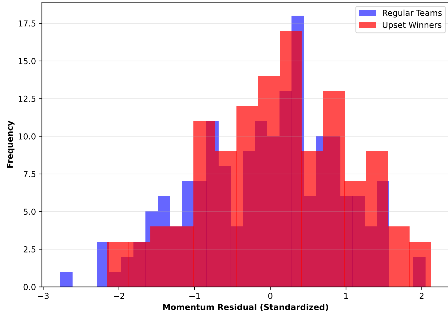
Momentum Distribution: Upset Winners vs Others
