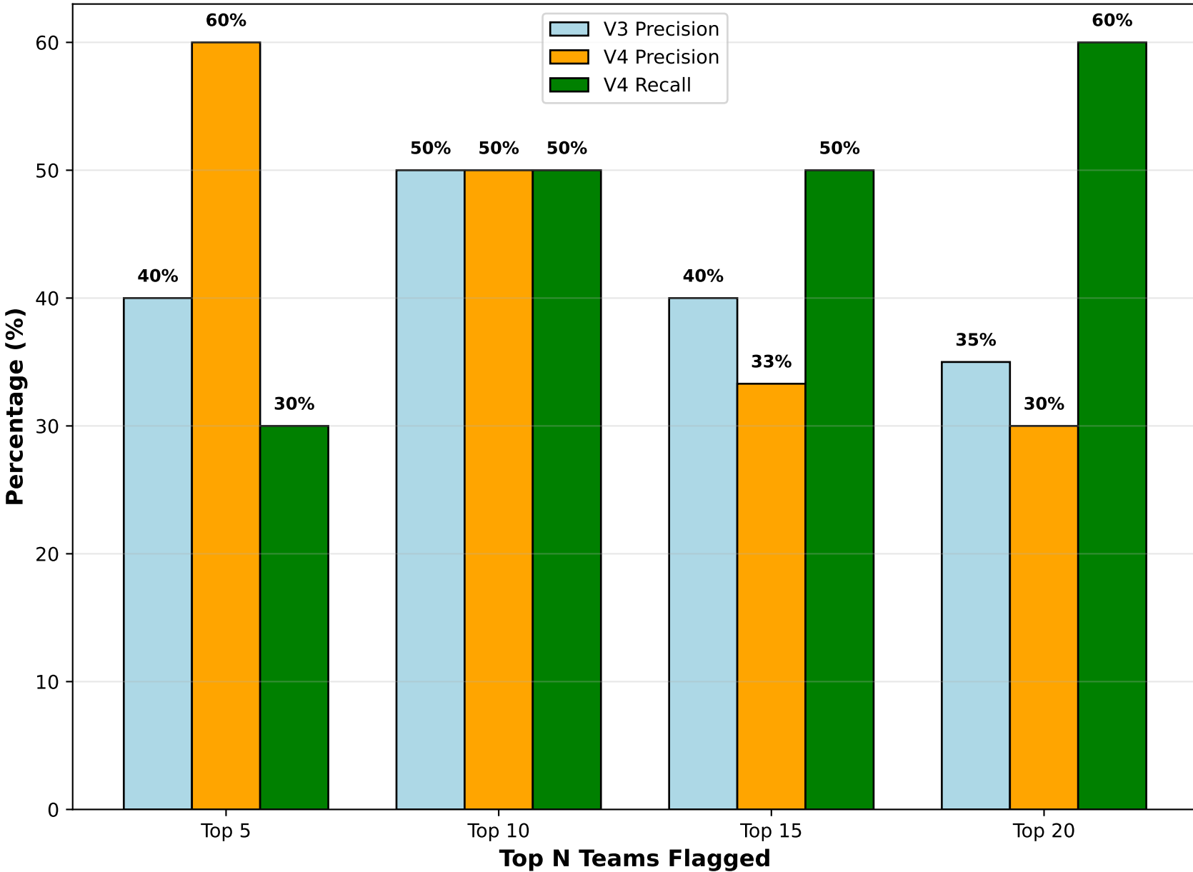
Model Performance: V4 Improvement
