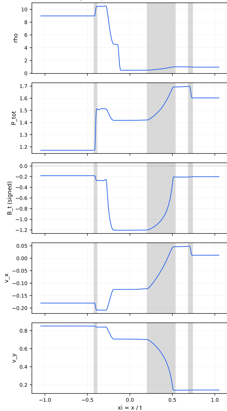
solved exactly: five planar waves — lane 853, B_n = +1.05
