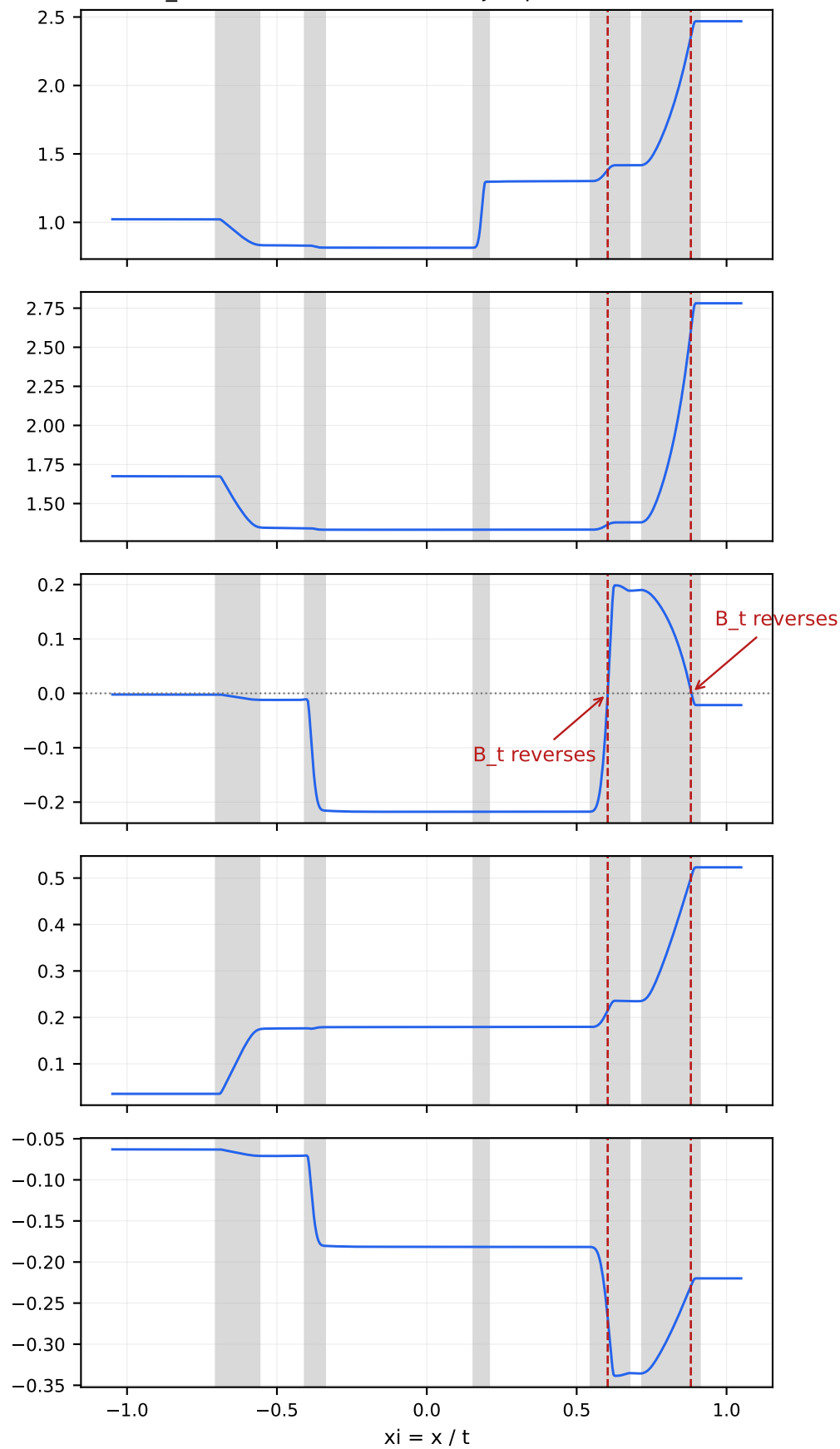
stubborn: B_t reverses where \rho and P jump — lane 431, B_n = +1.04
