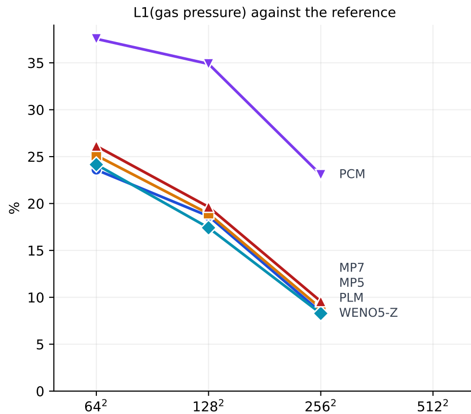
The rotor at t = 0.4 , HLLD flux, 5 reconstructions, against a 512^2 PLM (2nd) reference
