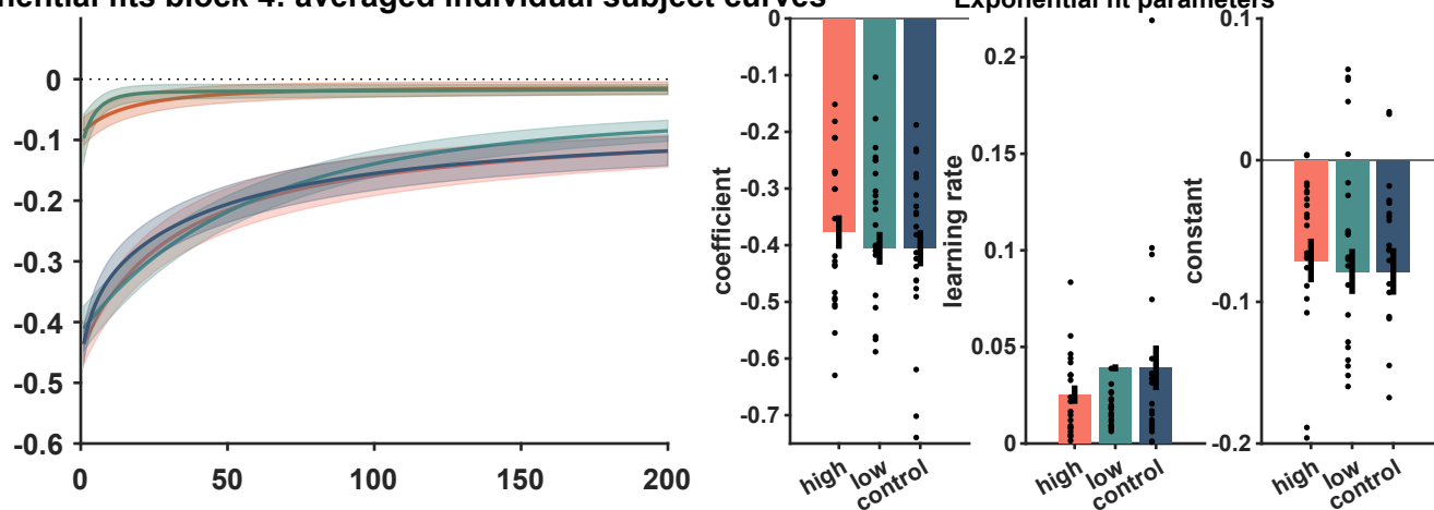
exponential fits block 4: averaged individual subject curves
