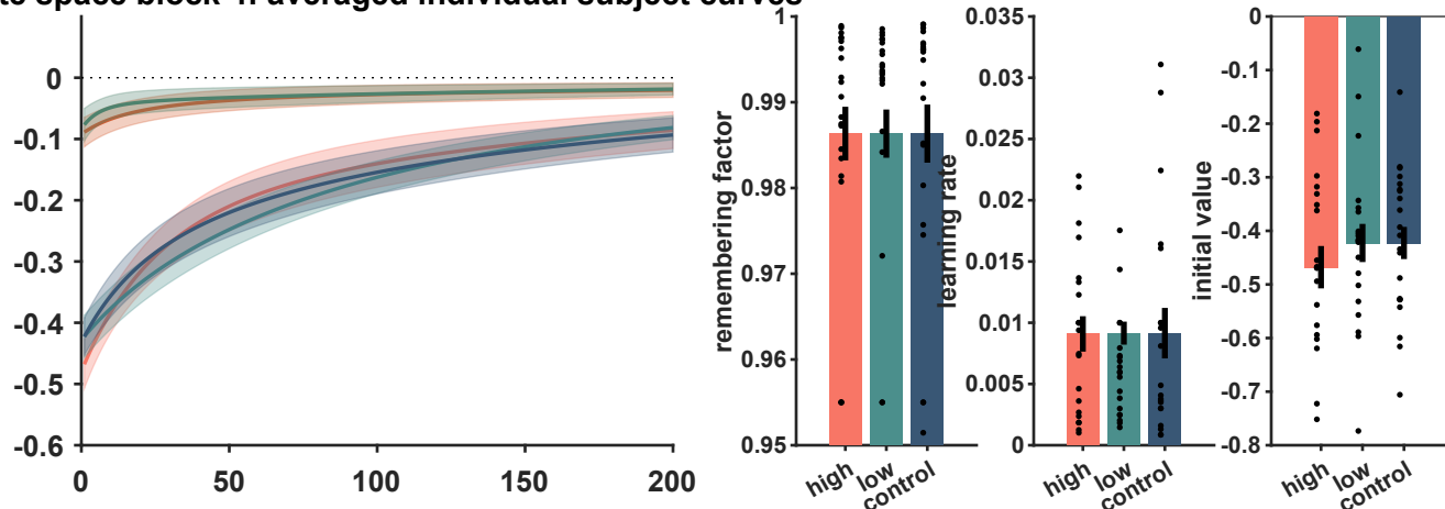
state space block 4: averaged individual subject curves
