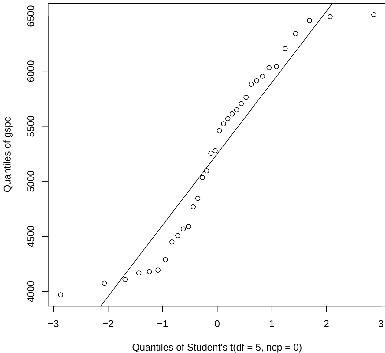
Student's t Q-Q Plot for gspc
