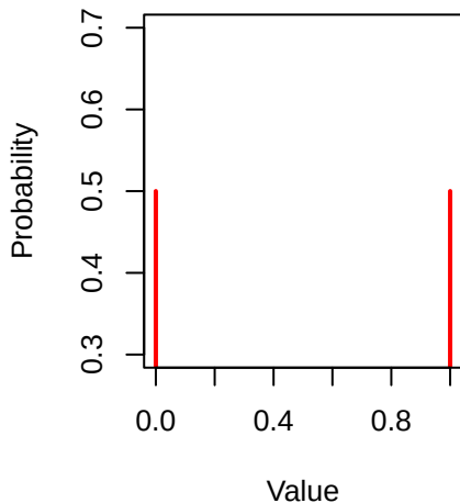
PMF of Binomial Distribution
