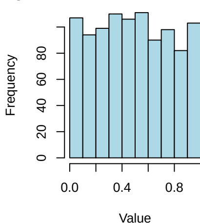
Histogram of Uniform Distribution Samples
