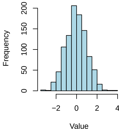
Histogram of Normal Distribution Samples
