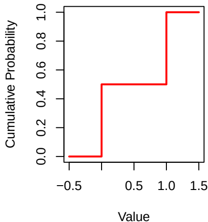
CDF of Binomial Distribution
