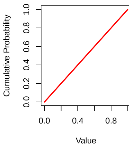
CDF of Uniform Distribution
