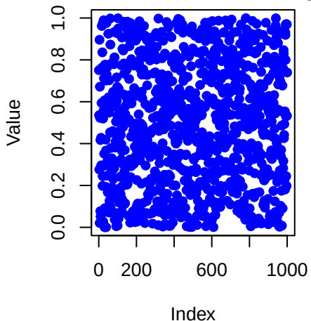
Uniform Distribution Samples
