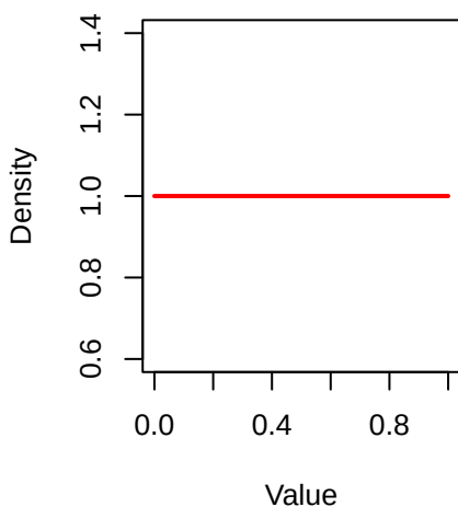
PDF of Uniform Distribution
