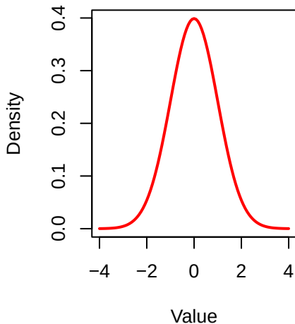
PDF of Normal Distribution
