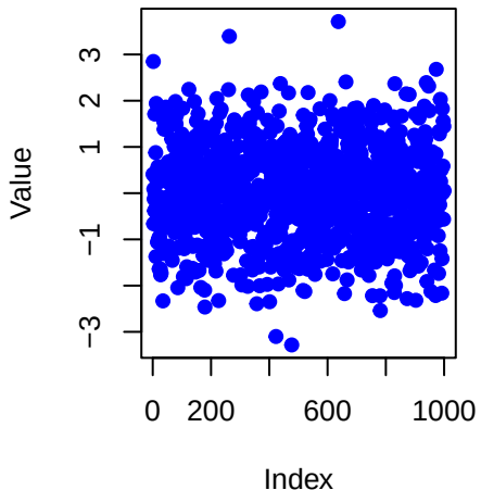
Normal Distribution Samples
