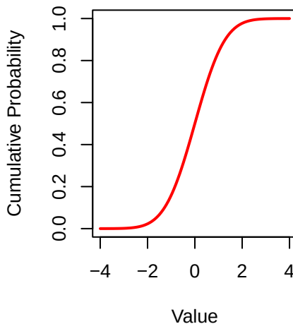
CDF of Normal Distribution
