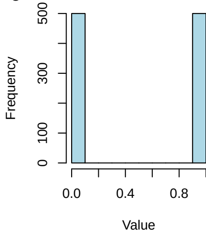
Histogram of Binomial Distribution Samples
