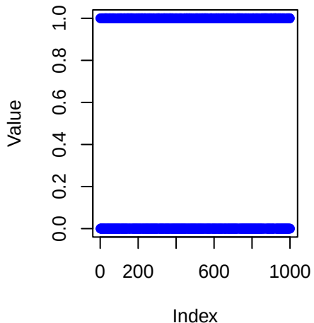
Binomial Distribution Samples
