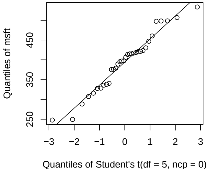
Student's t Q-Q Plot for msft
