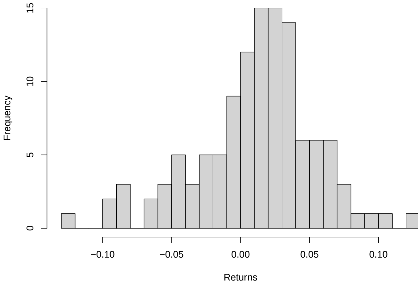
X.gspc – Histogram of Returns
