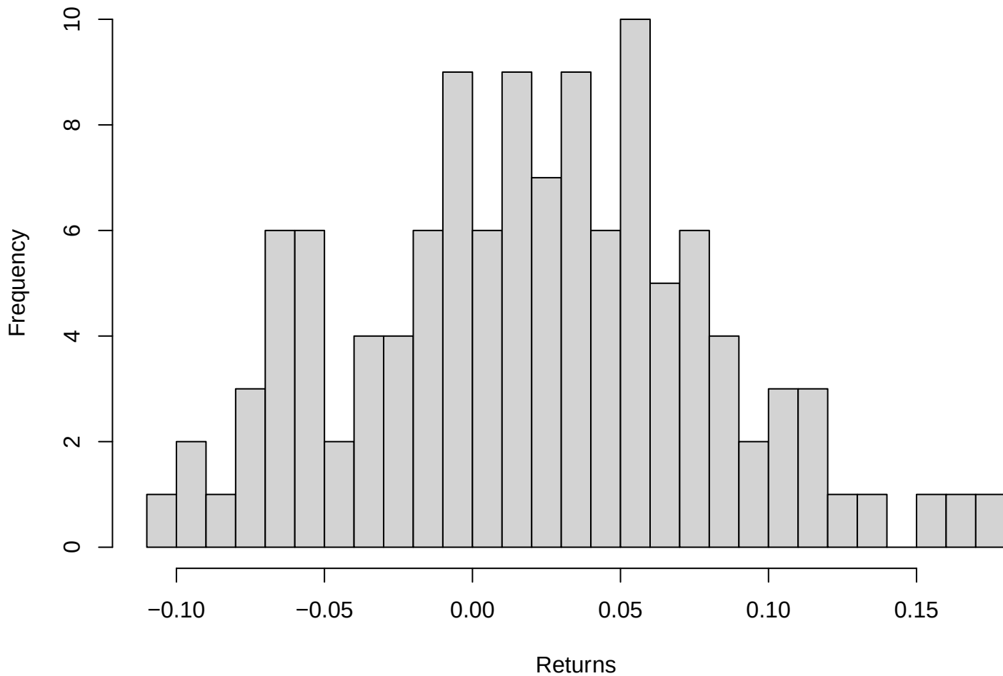
msft – Histogram of Returns
