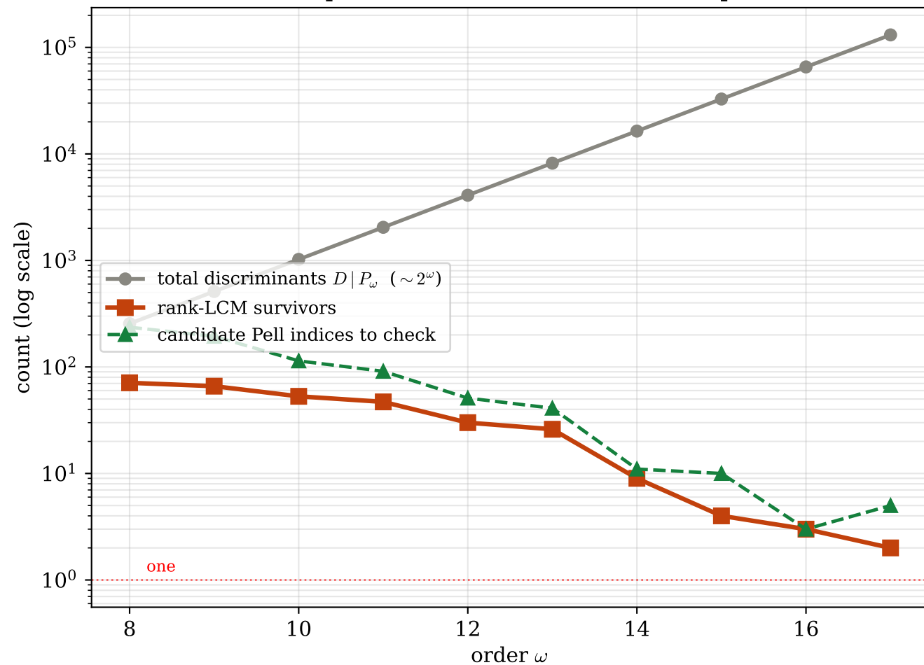
Search space vanishes while D -count explodes
