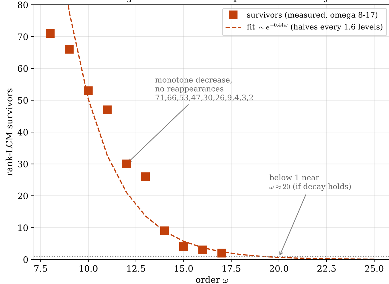
The signal: survivors collapse monotonically
