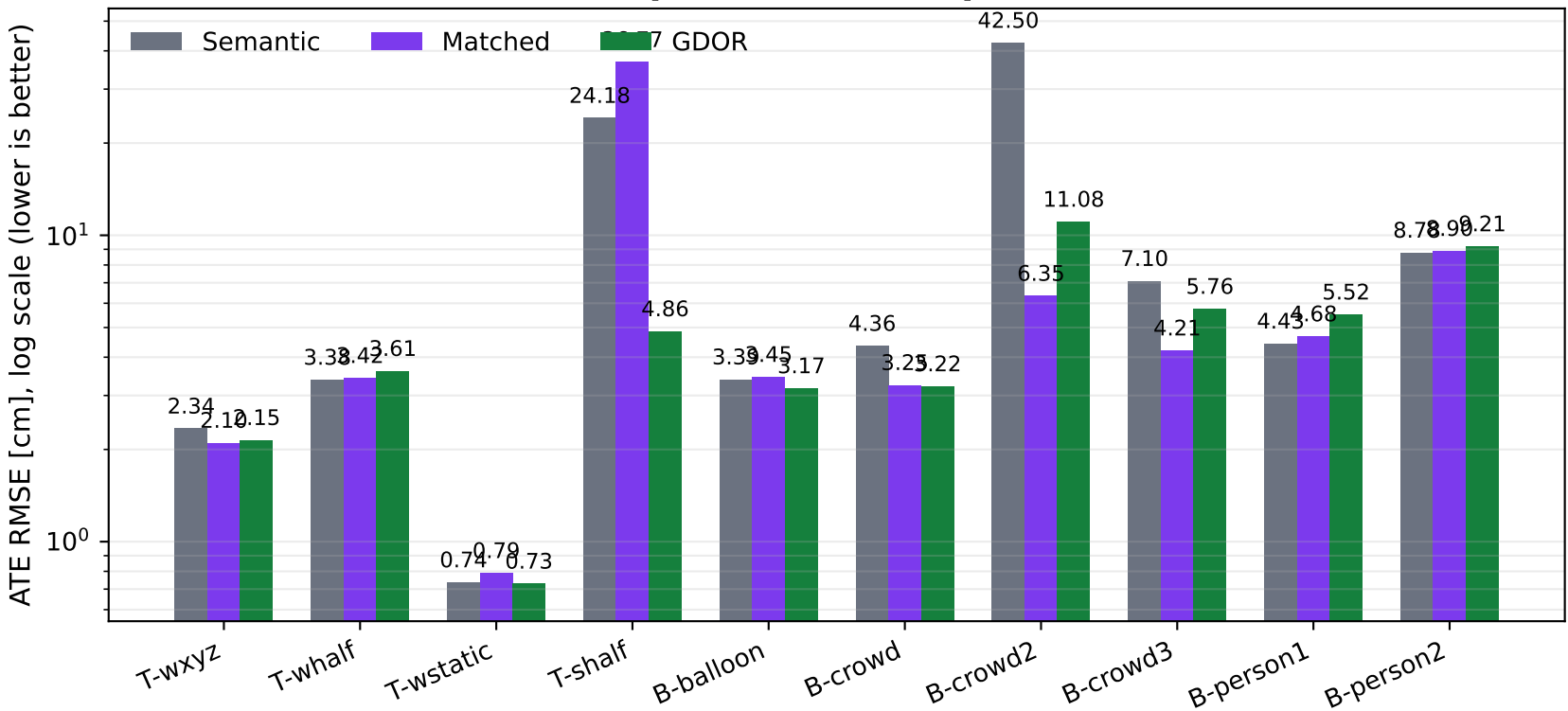
DYN-19 main comparison: ten sequences, three seeds
