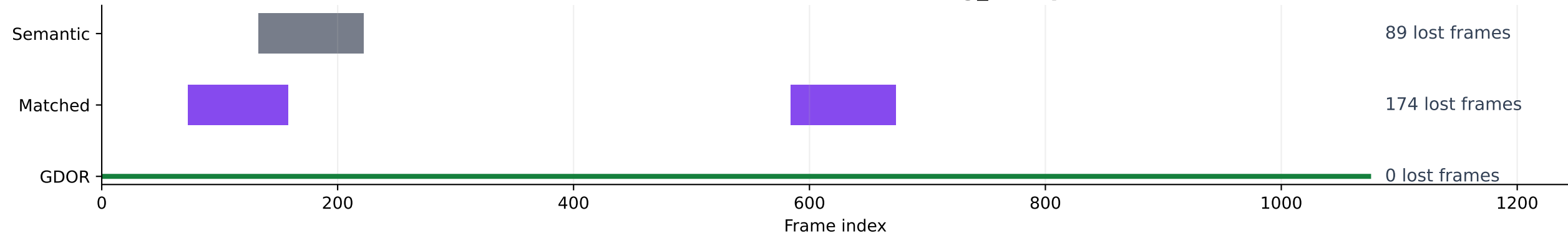
Per-frame failure intervals on TUM sitting_halfsphere, seed 0
