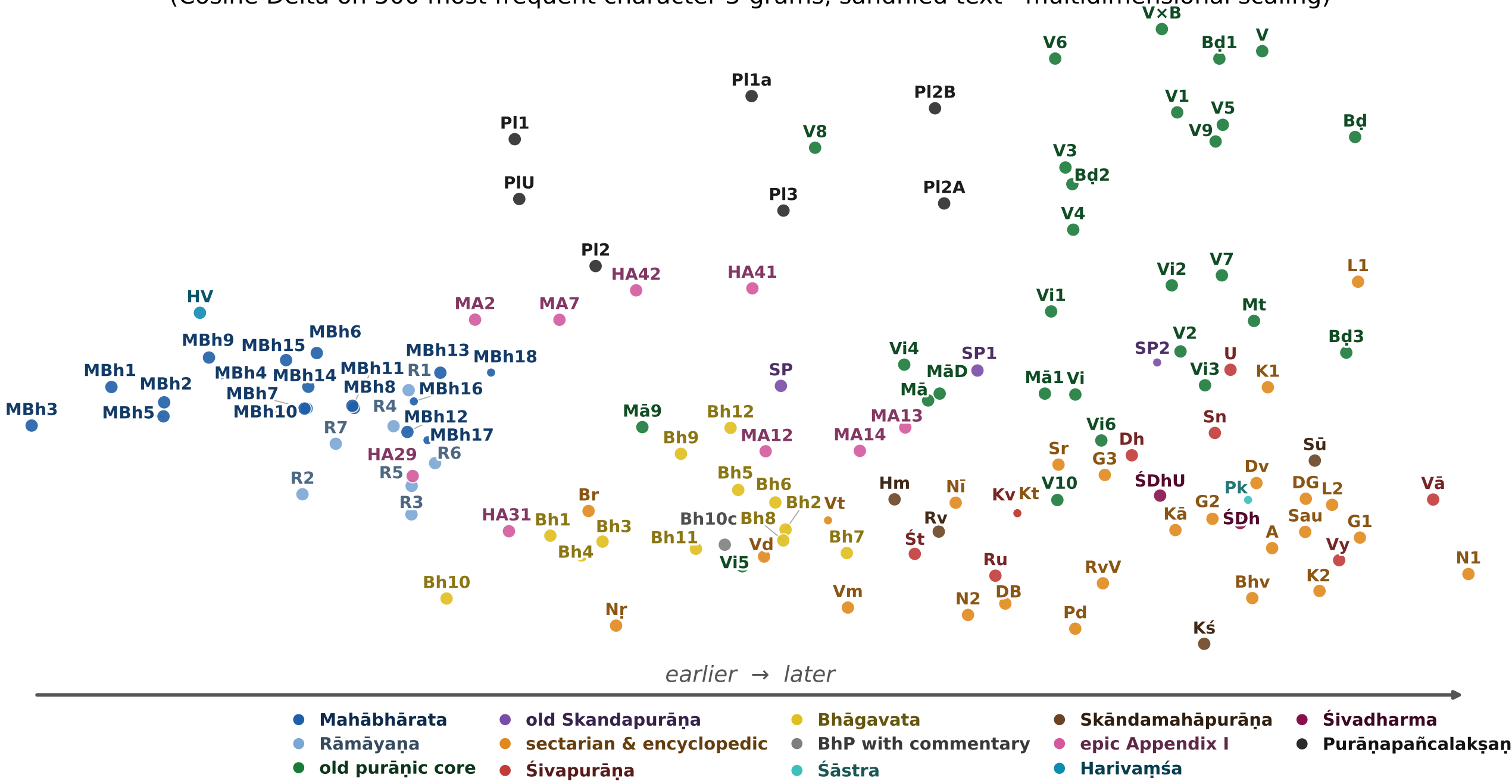
127 epic and purāṇic texts, arranged only by counted linguistic habits (Cosine Delta on 500 most frequent character 3-grams, sandhied text · multidimensional scaling)
