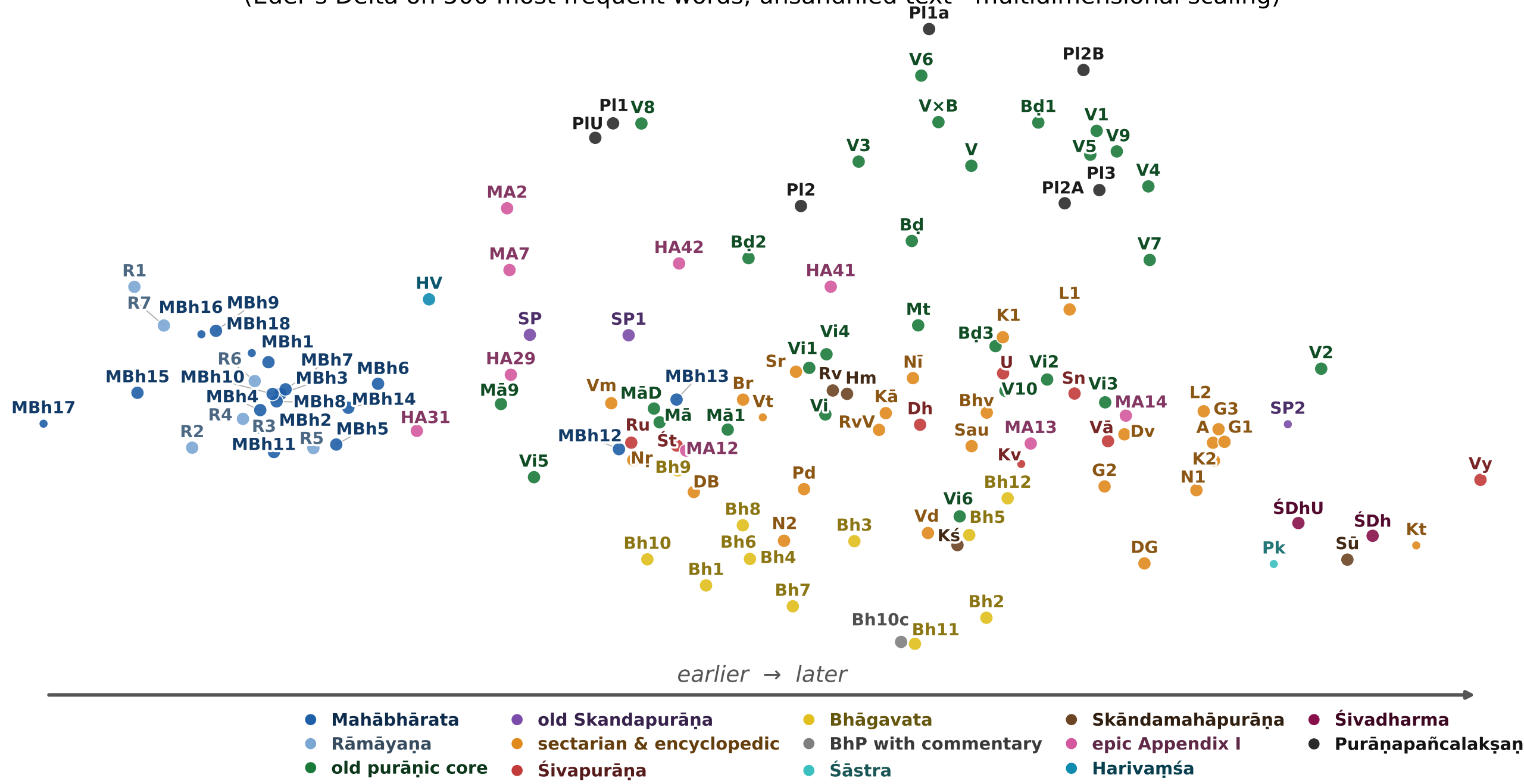
127 epic and purāṇic texts, arranged only by counted linguistic habits (Eder's Delta on 500 most frequent words, unsandhied text · multidimensional scaling)
