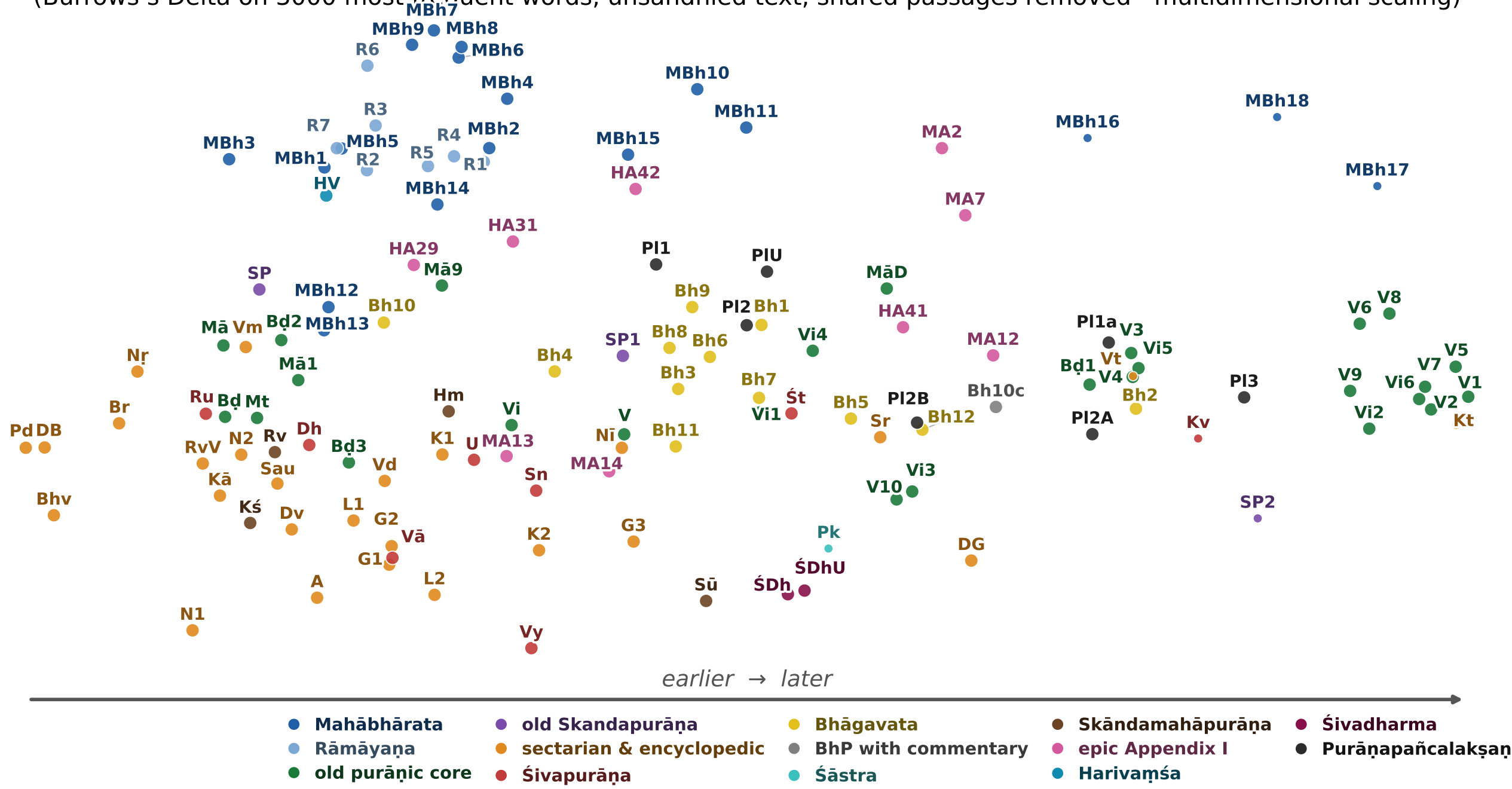
126 epic and purāṇic texts, arranged only by counted linguistic habits (Burrows's Delta on 3000 most frequent words, unsandhied text, shared passages removed · multidimensional scaling)
