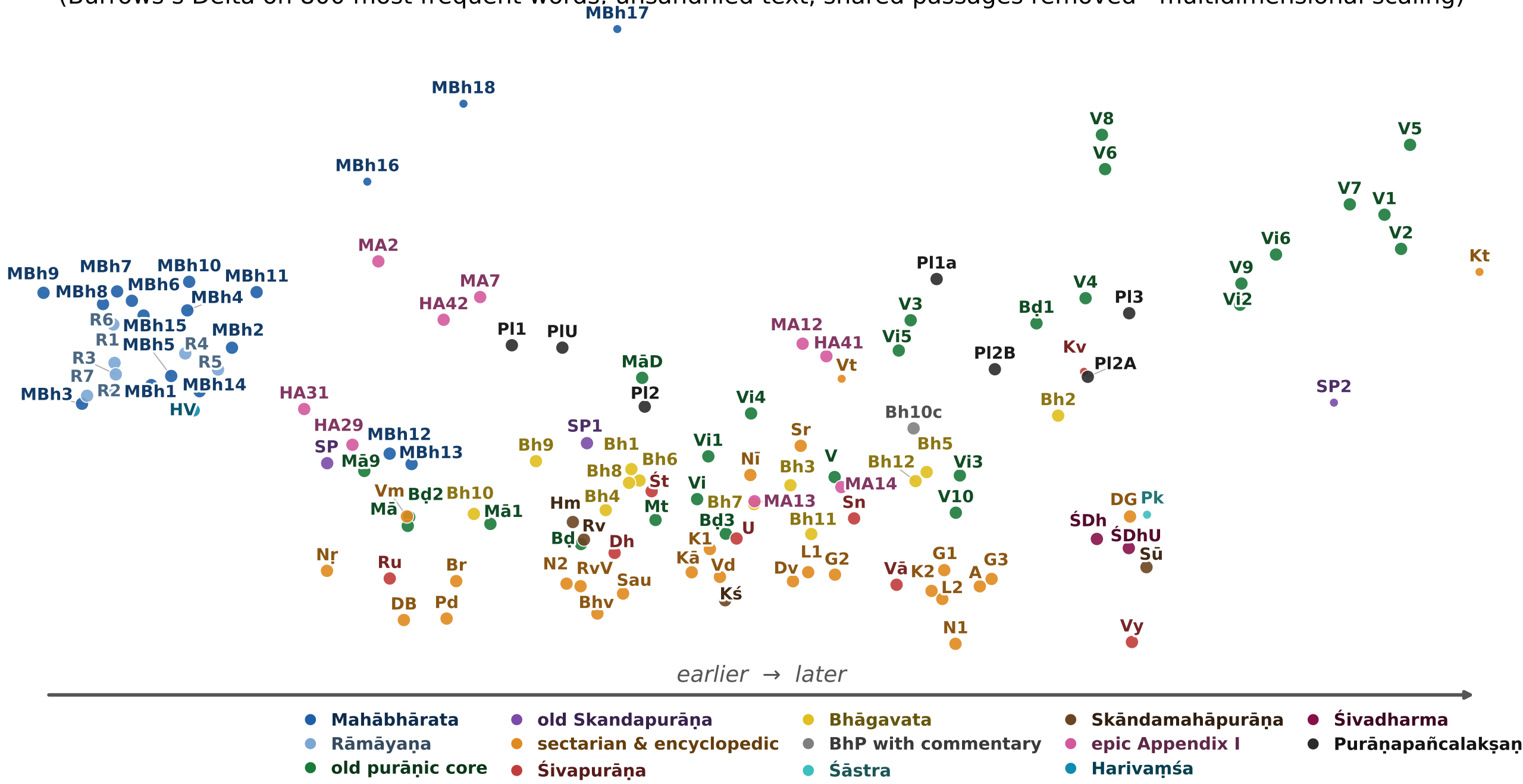
126 epic and purāṇic texts, arranged only by counted linguistic habits (Burrows's Delta on 800 most frequent words, unsandhied text, shared passages removed · multidimensional scaling)
