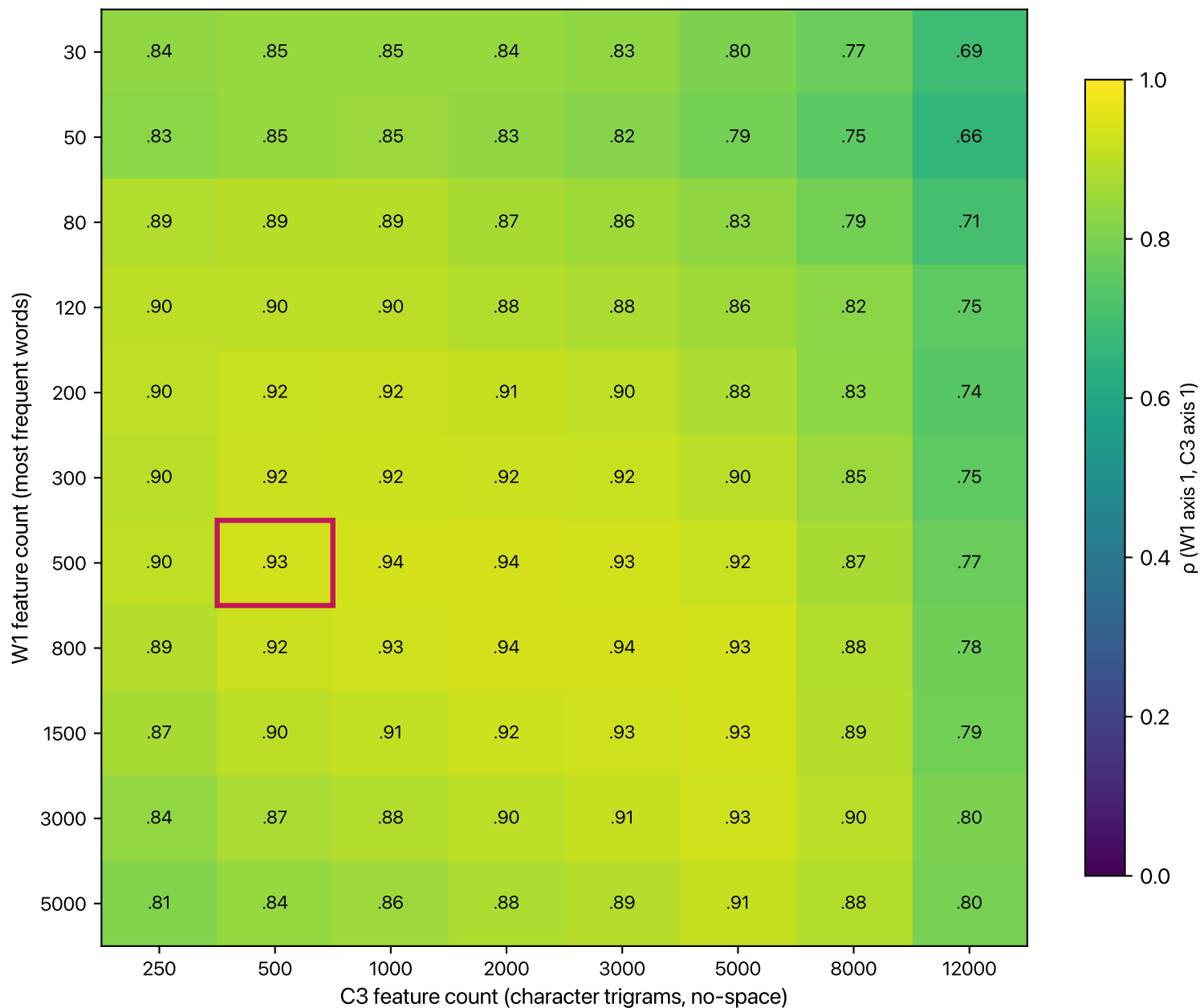
Cross-lens axis-1 agreement (Spearman \rho ), 126 units, cleaned build adopted setting 500 \times 500 outlined
