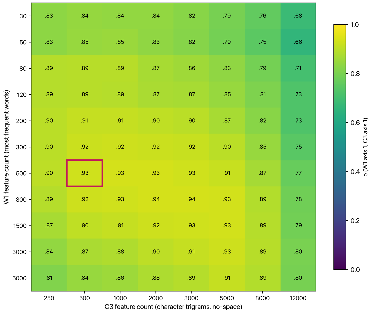
Cross-lens axis-1 agreement (Spearman \rho ), 126 units, cleaned build adopted setting 500 × 500 outlined
