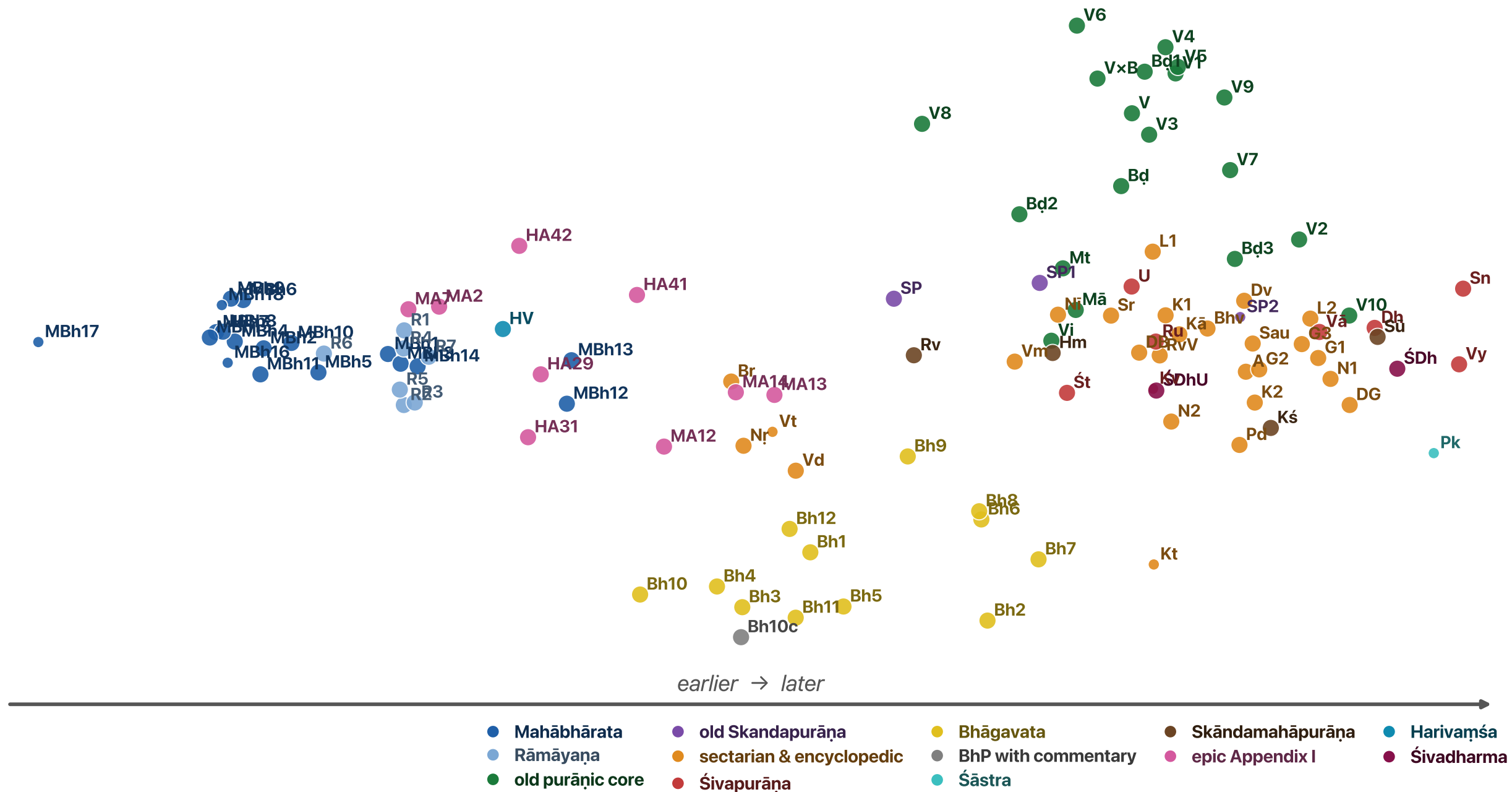
111 epic and purāṇic texts, arranged only by counted linguistic habits (Manhattan distance on 5000 most frequent character 3-grams, sandhied text · multidimensional scaling)
