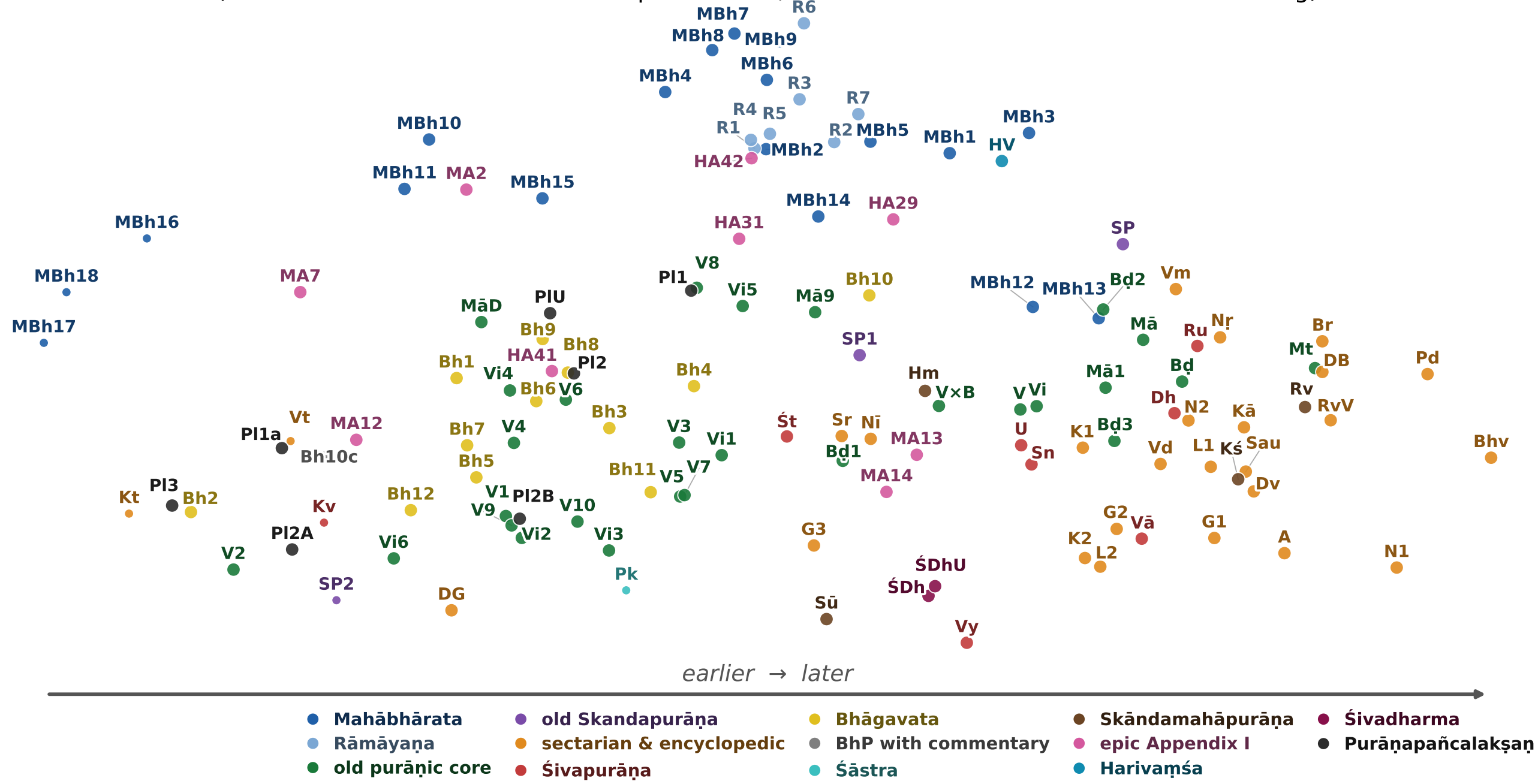
127 epic and purāṇic texts, arranged only by counted linguistic habits (Burrows's Delta on 5000 most frequent words, unsandhied text · multidimensional scaling)
