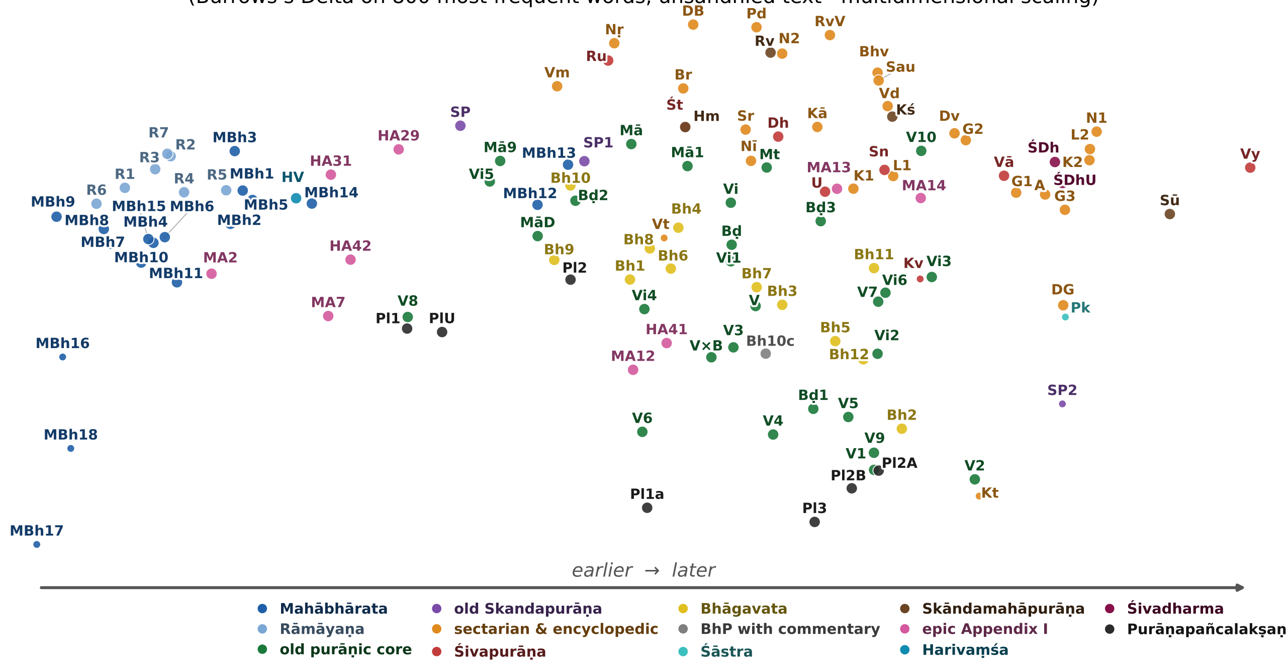
127 epic and purāṇic texts, arranged only by counted linguistic habits (Burrows's Delta on 800 most frequent words, unsandhied text · multidimensional scaling)
