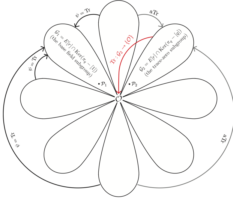
Figure 1: The behaviour of the trace and anti-trace maps on E[r] (from [Cos12]).
