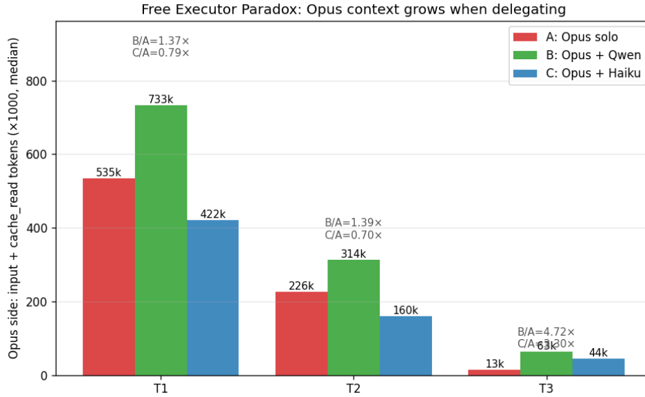
Figure 4: Free-executor paradox visualized. Each bar is the success-only median of Opus-side ( input + cache_read ) tokens for the corresponding task. Even though arm B’s executor (Qwen) is free at the token meter, the orchestrator’s own context (green bars) is consistently larger than running Opus solo (red). Multipliers in grey annotate the B-over-A and C-over-A ratios per task.
