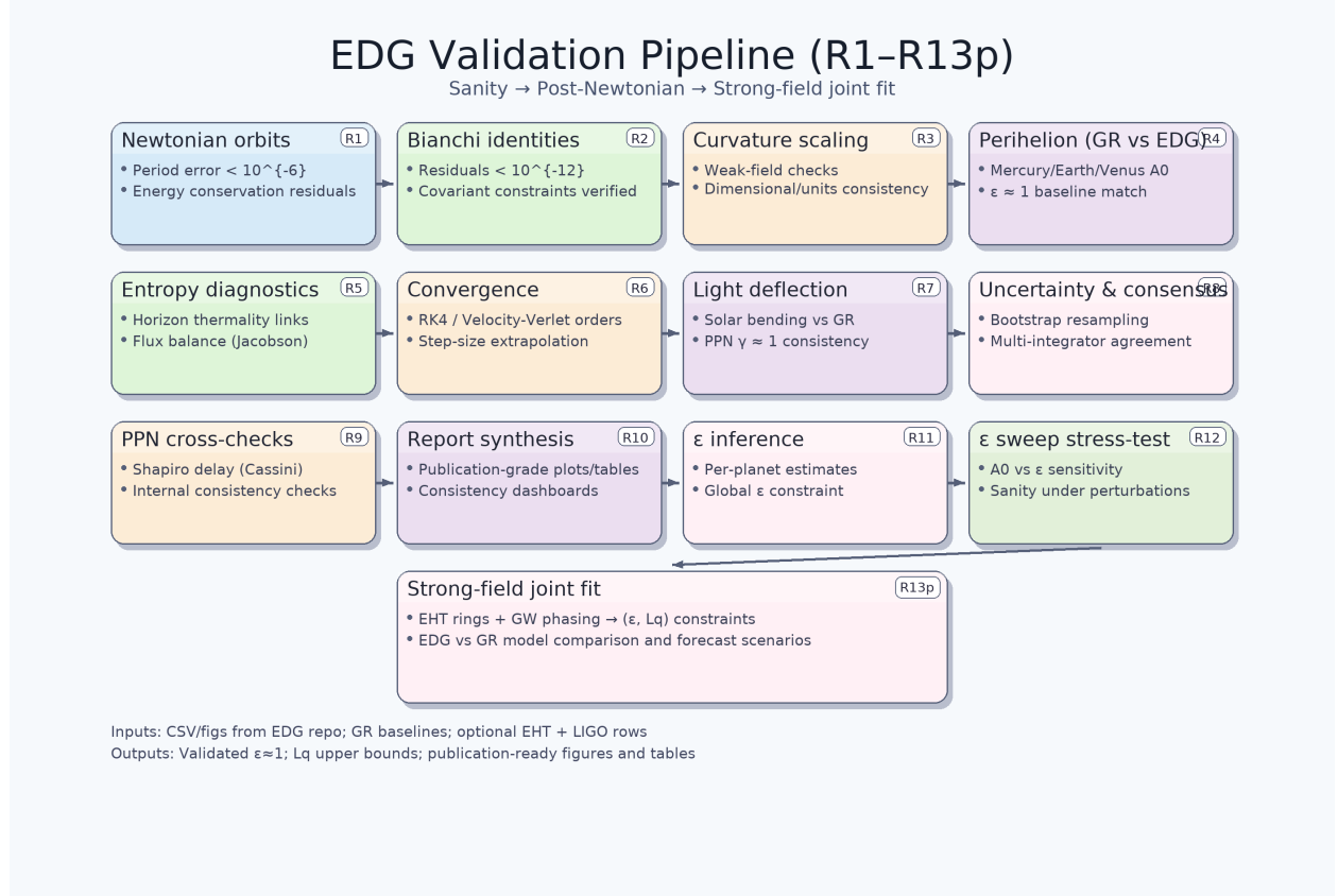
Figure 3: EDG validation pipeline (R1–R13p): sanity \rightarrow post-Newtonian \rightarrow strong-field joint fit.
