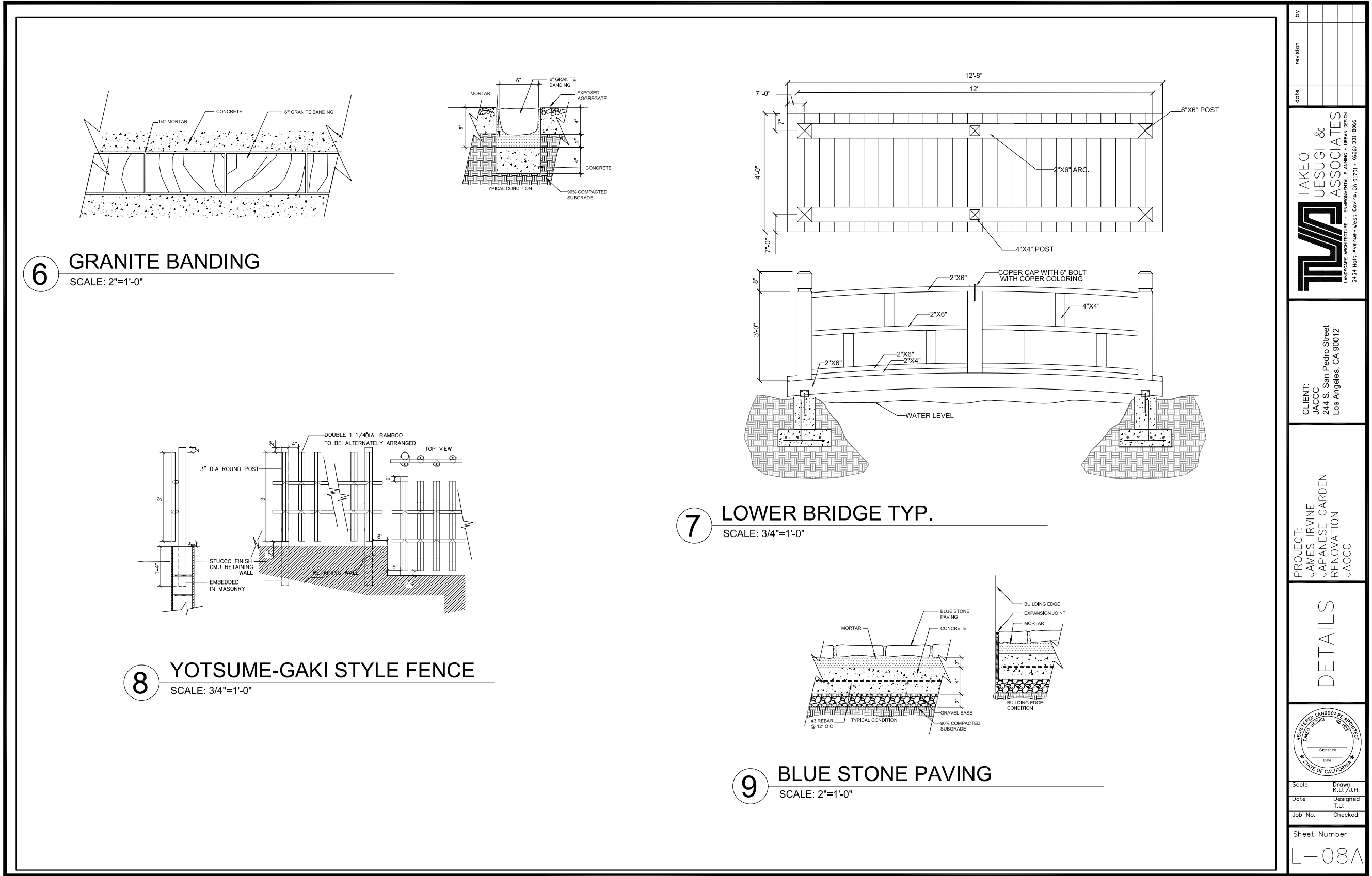
Construction documents detailing the construction of the JACCC garden elements.
