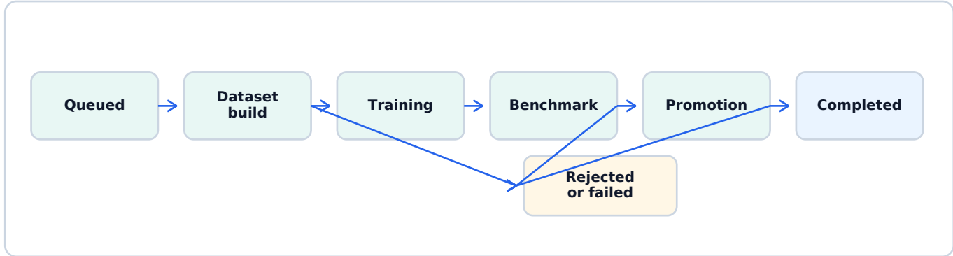
Figure 3. Guarded dream-cycle state machine. Training completion alone never changes the active adapter.
