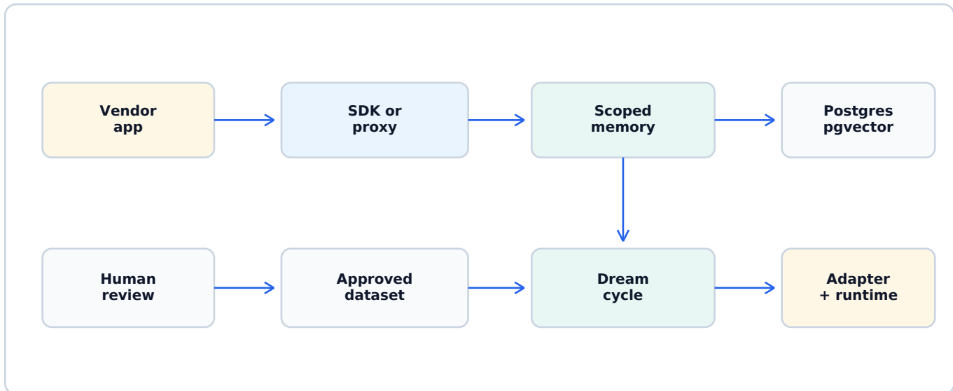
Figure 1. DreamCycle system map. The add-on owns memory, review, dataset creation, local cycle orchestration, and adapter state while the vendor keeps the UI and runtime.
