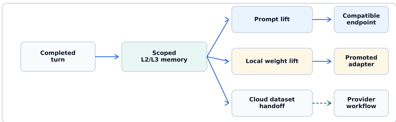
Figure 2. Three behavior-improvement layers: prompt lift, local weight lift, and cloud dataset handoff.
