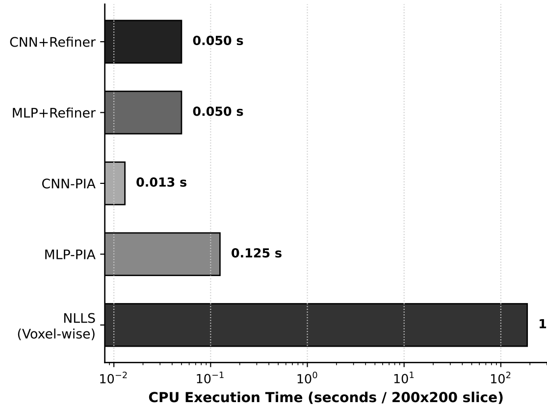
CPU Latency (Intel Core i7)
