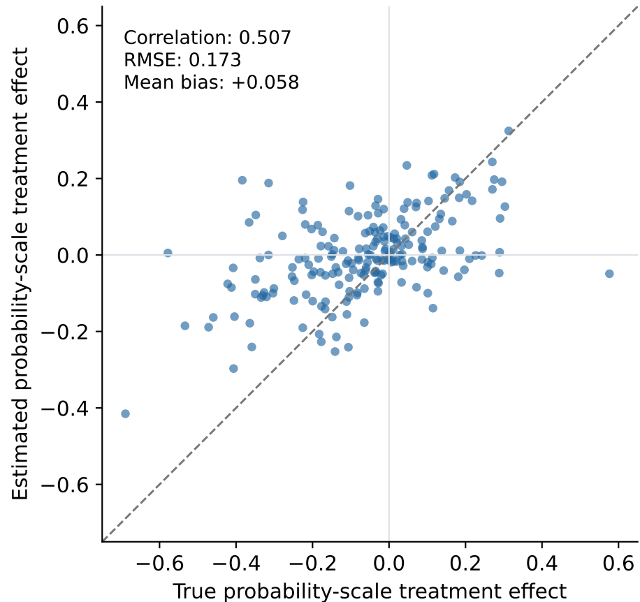
Elastic net
