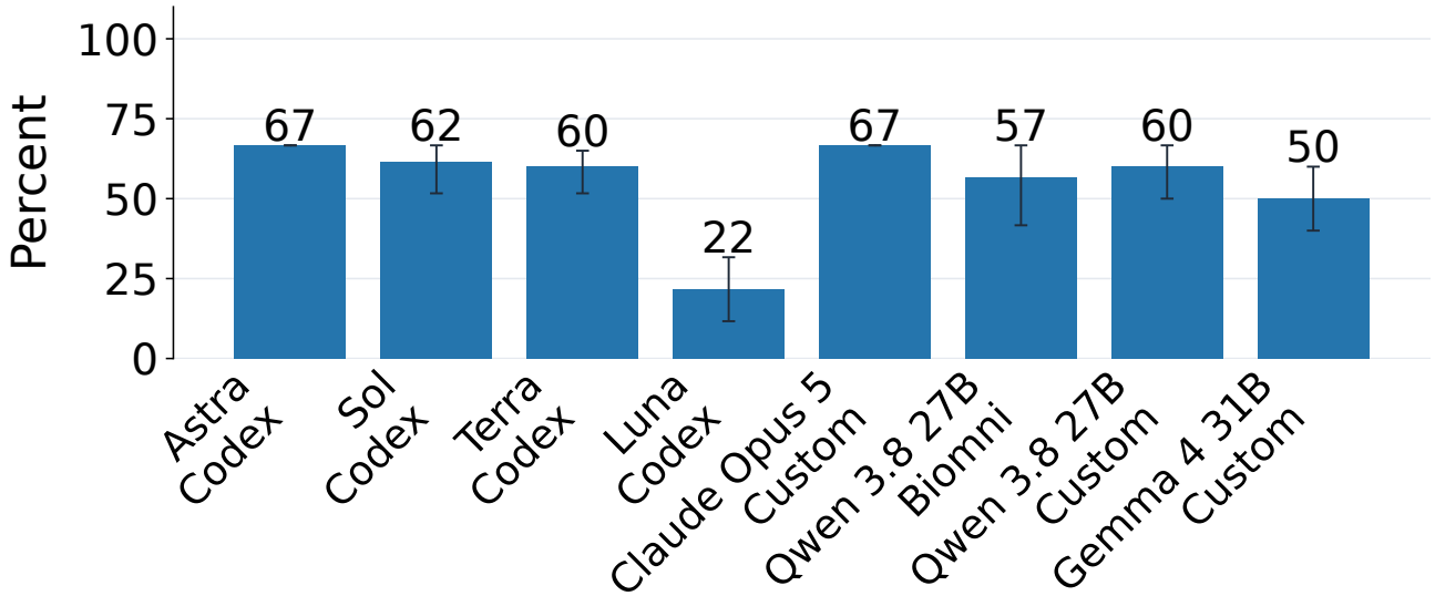
Surprising · Unmasked
