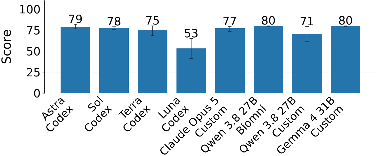
Surprising · Masked
