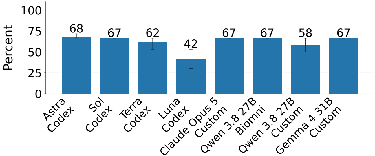
Surprising · Masked
