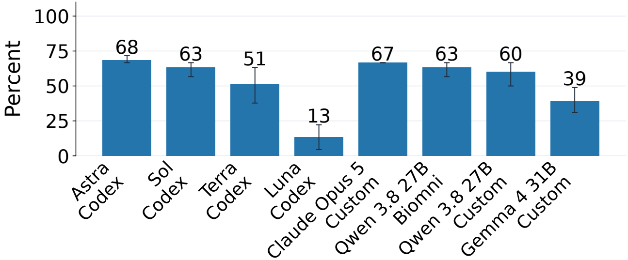
Surprising · Unmasked
