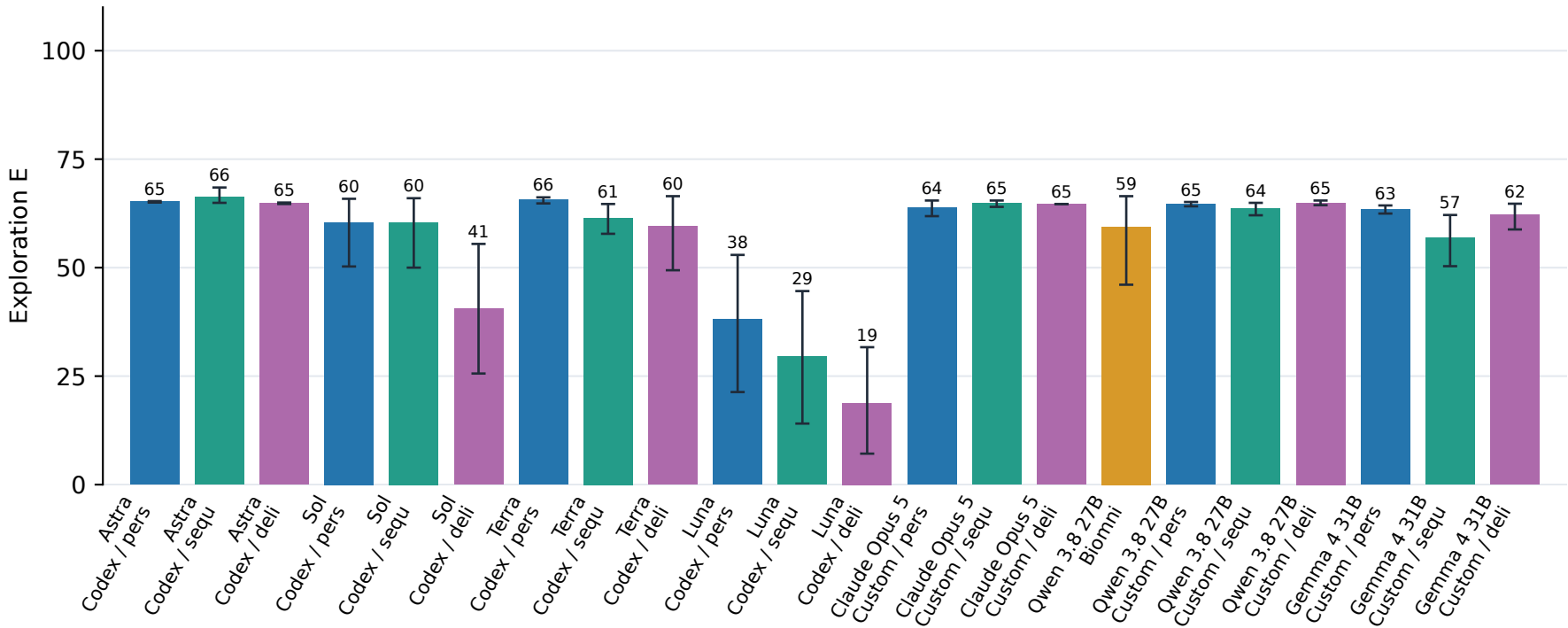
Surprising · Unmasked
