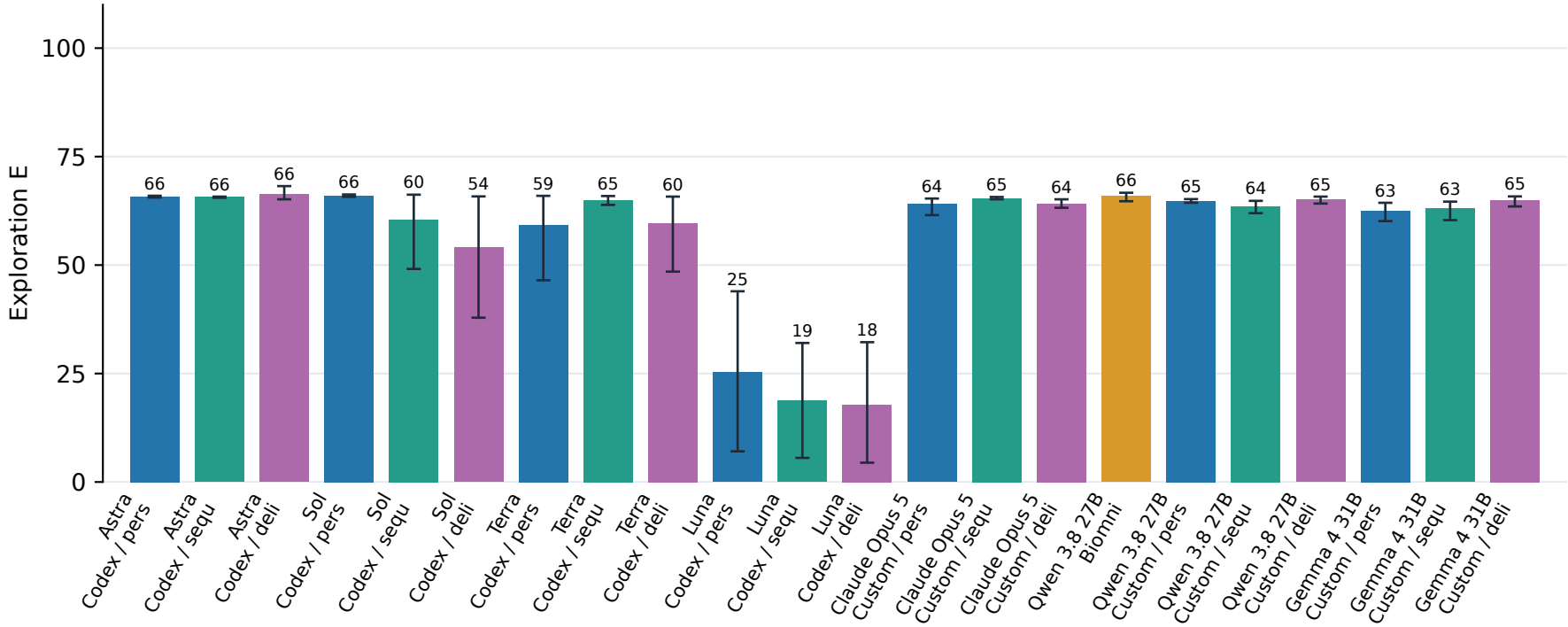
Expected · Unmasked
