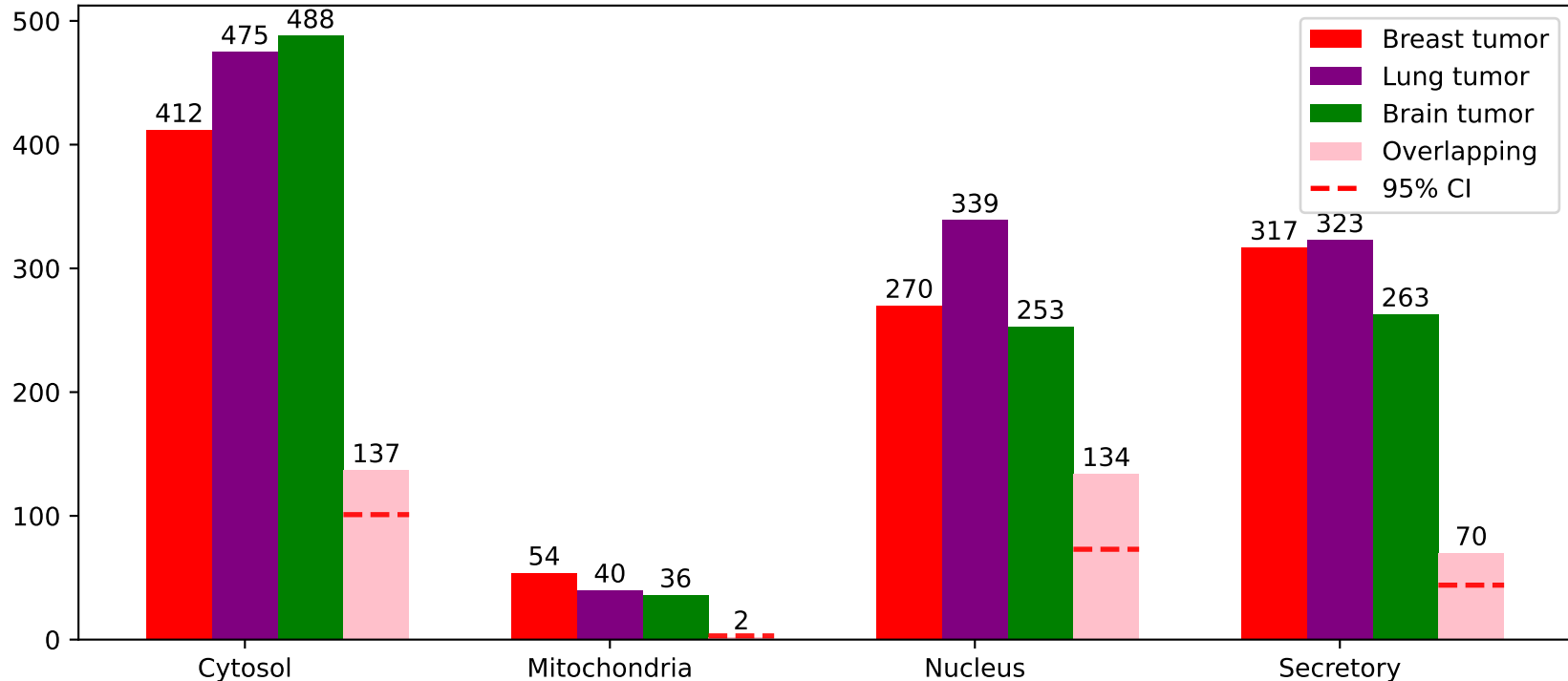
Correct Predictions
