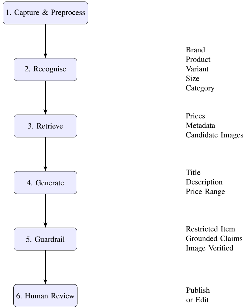
Fig. 1. Snap-to-Sell end-to-end architecture. A product image passes through preprocessing, multimodal recognition, retrieval grounding, listing generation, responsible-AI validation, and human review before publication.
