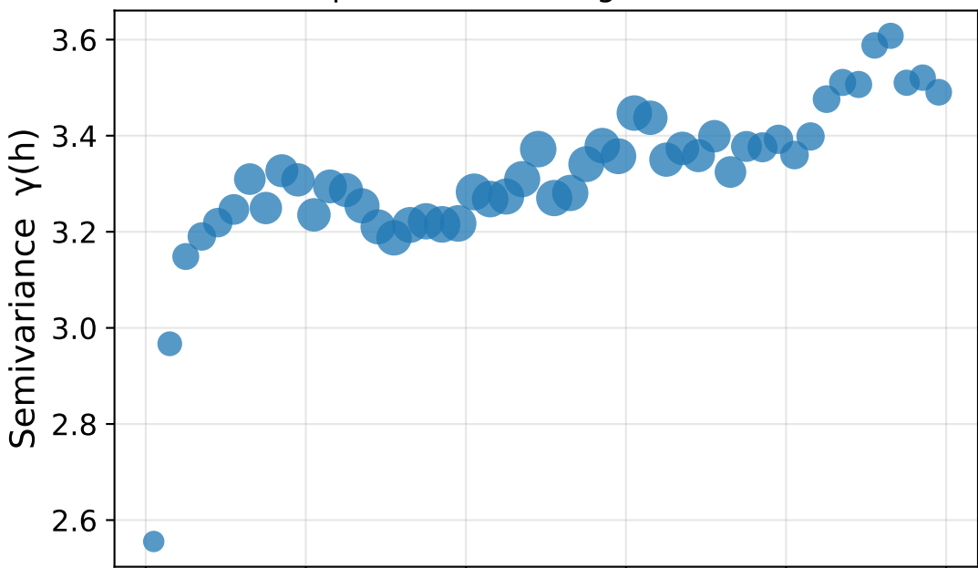
Empirical Semivariogram — 2020
