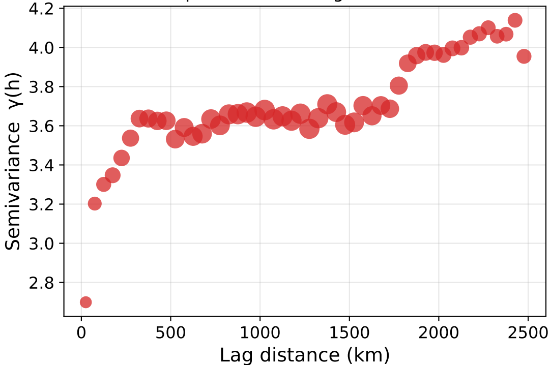
Empirical Semivariogram — 2022
