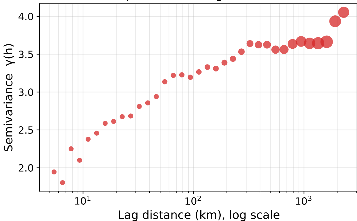
Empirical Semivariogram — 2022
