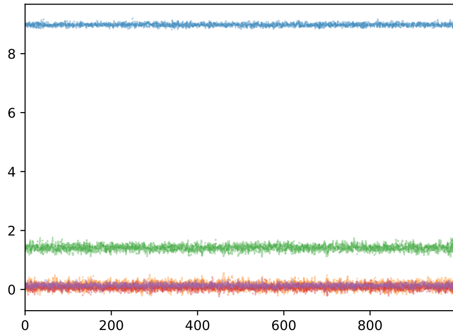
beta
