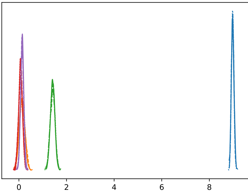
beta
