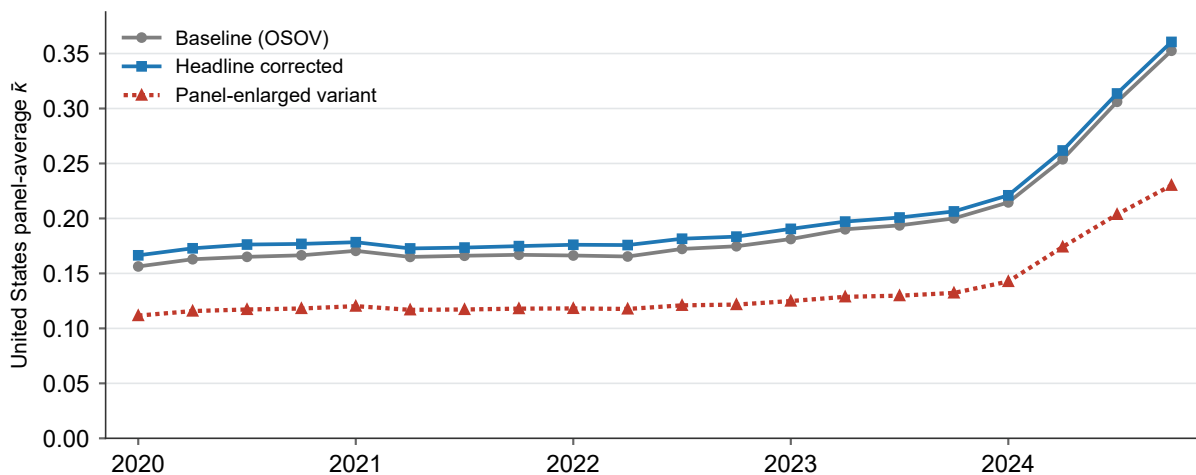
Figure 6: United States panel-average \bar{\kappa} under the three lenses, 2020Q1–2024Q4
