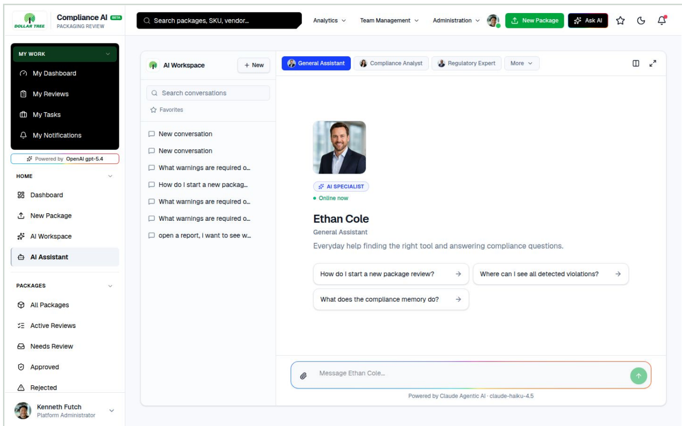
AI Workspace — chat with a specialist grounded in live platform data.
