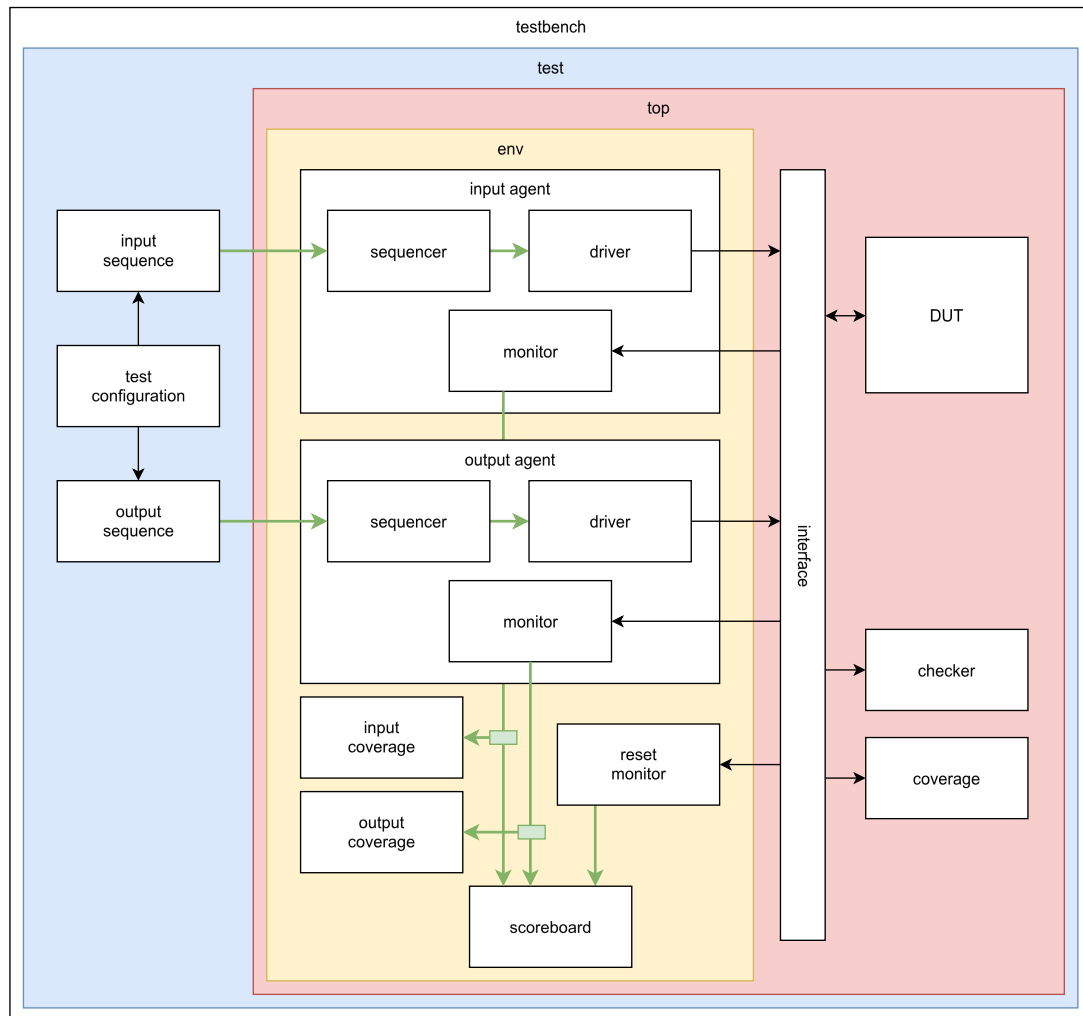
Figure 3.1: UVM architecture of the DUT
