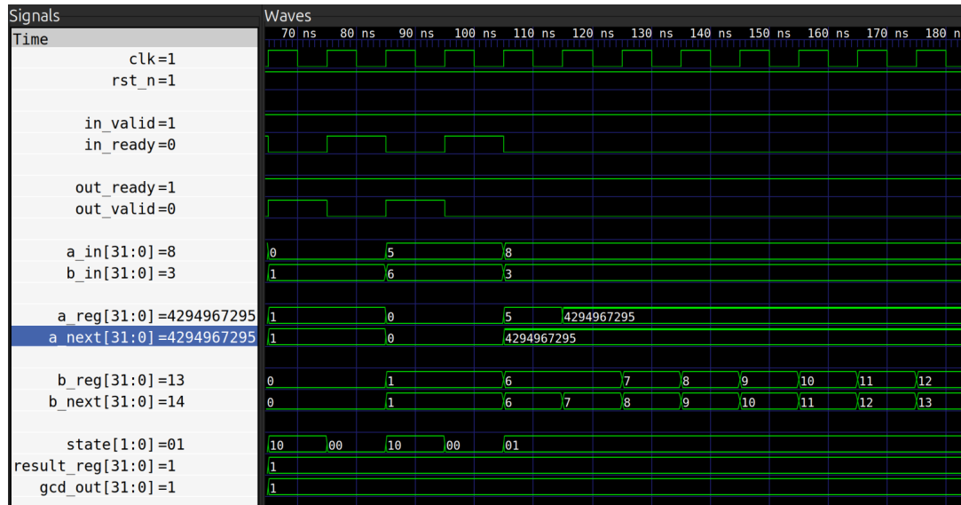
Figure 4.2: Wave of Bug in the DUT
