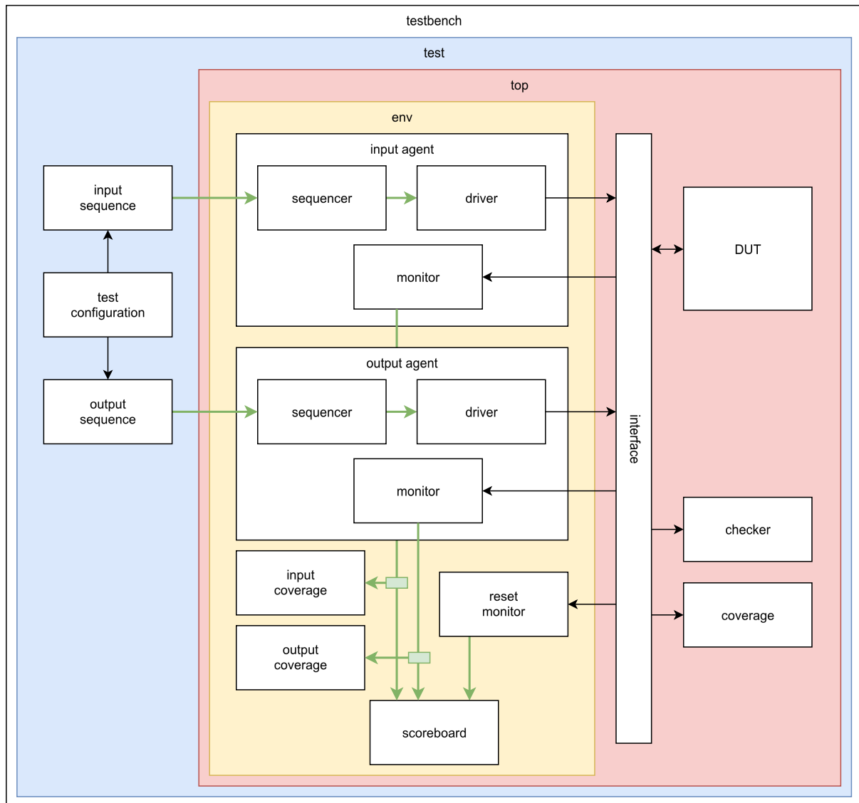
Figure 3.1: UVM architecture of the DUT
