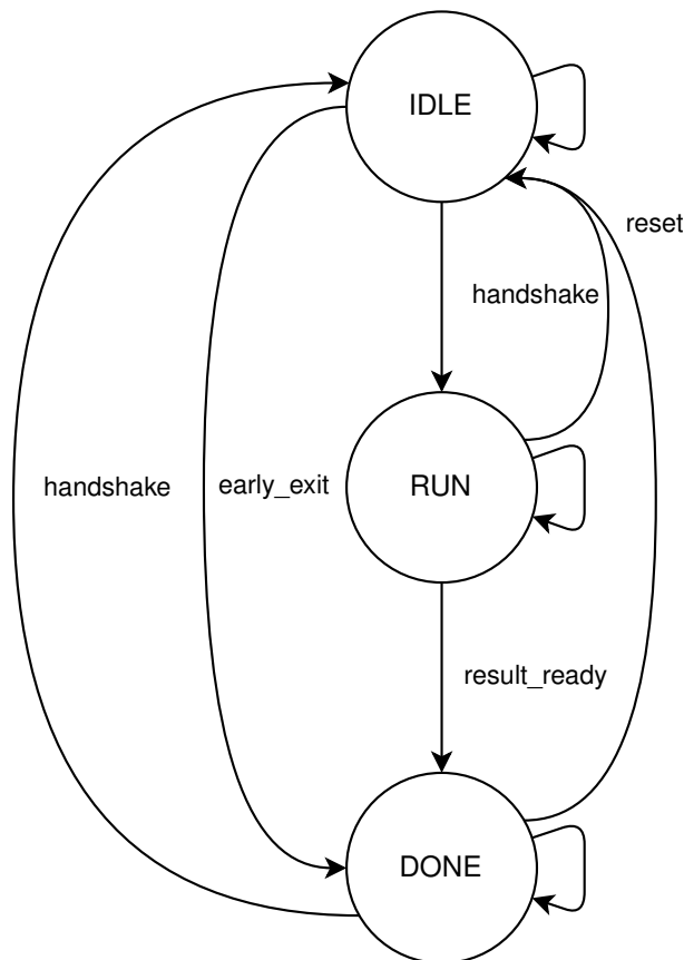
Figure 2.1: Finite State machine of the DUT
